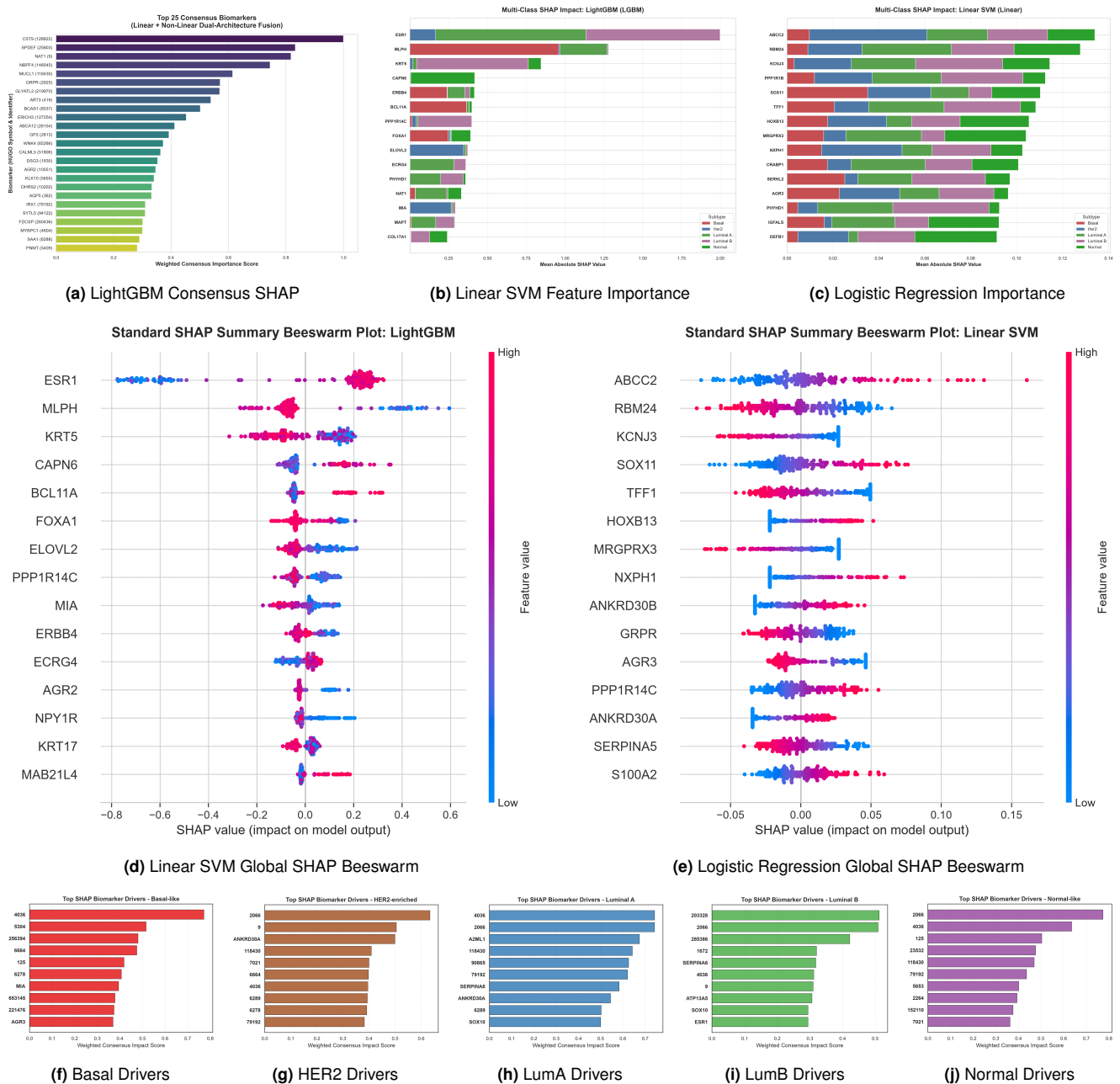
Figure 14. Multi-Model Explainable AI (SHAP) Biomarker Attribution, Global Beeswarm Distributions, and Subtype Driver Signatures.
