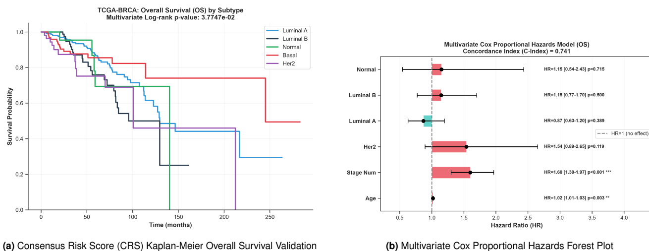
Figure 11. Consensus Risk Score (CRS) Prognostic Overall Survival Stratification and Cox Hazard Ratios.
