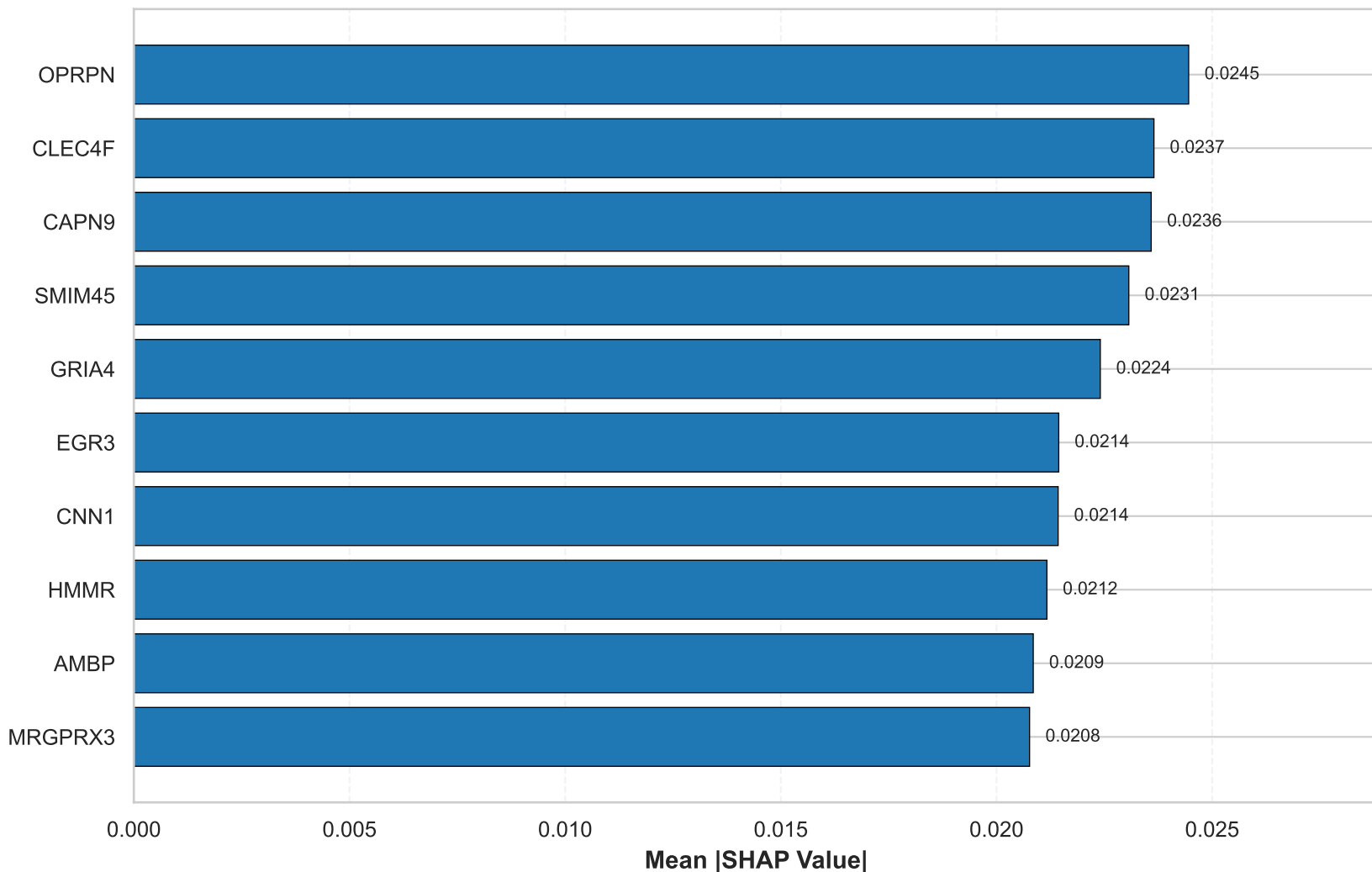
Subtype: NORMAL Logistic Regression SHAP Feature Importance
