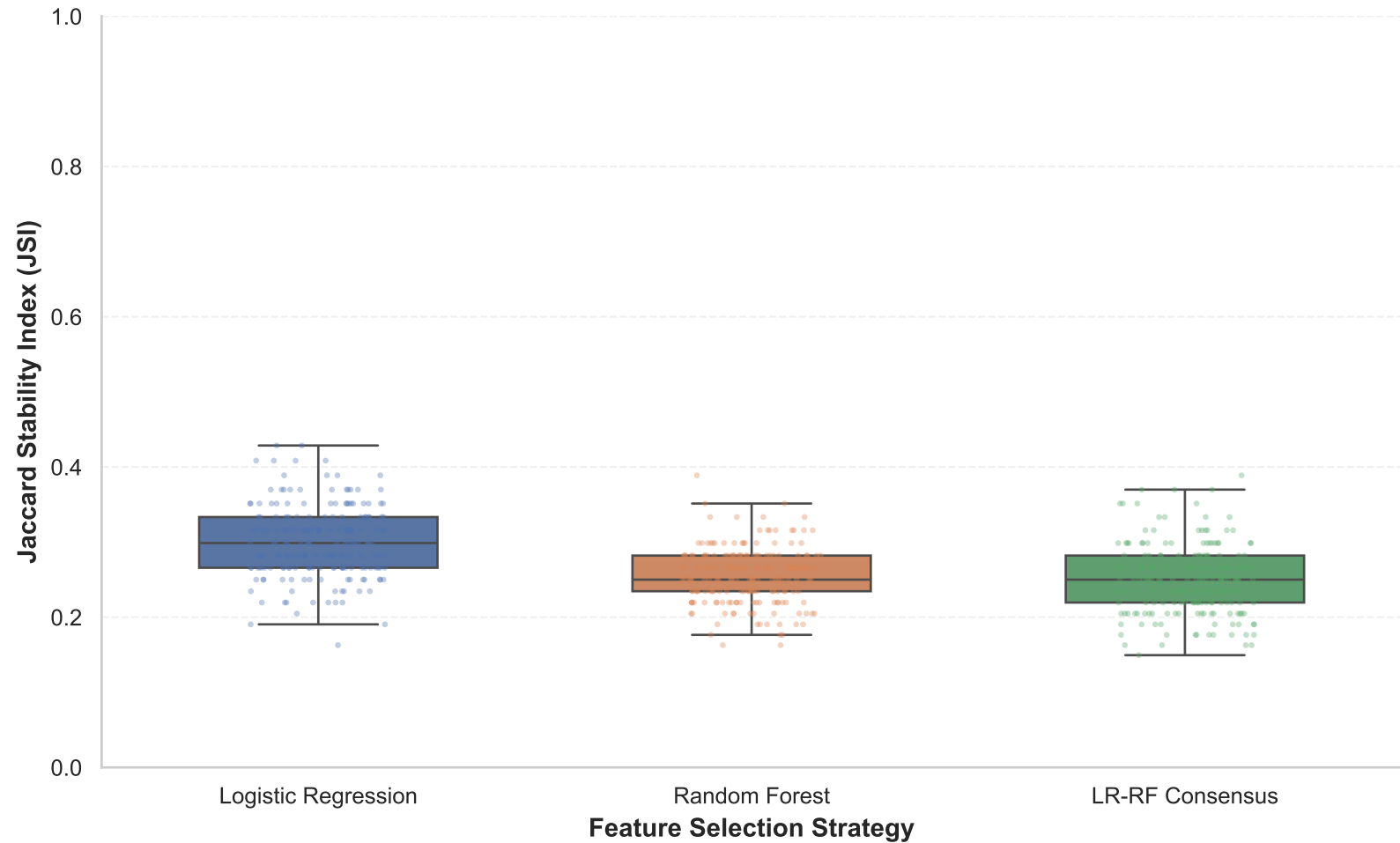
Feature Selection Stability Across 20 Stratified Resamples (Top-50)
