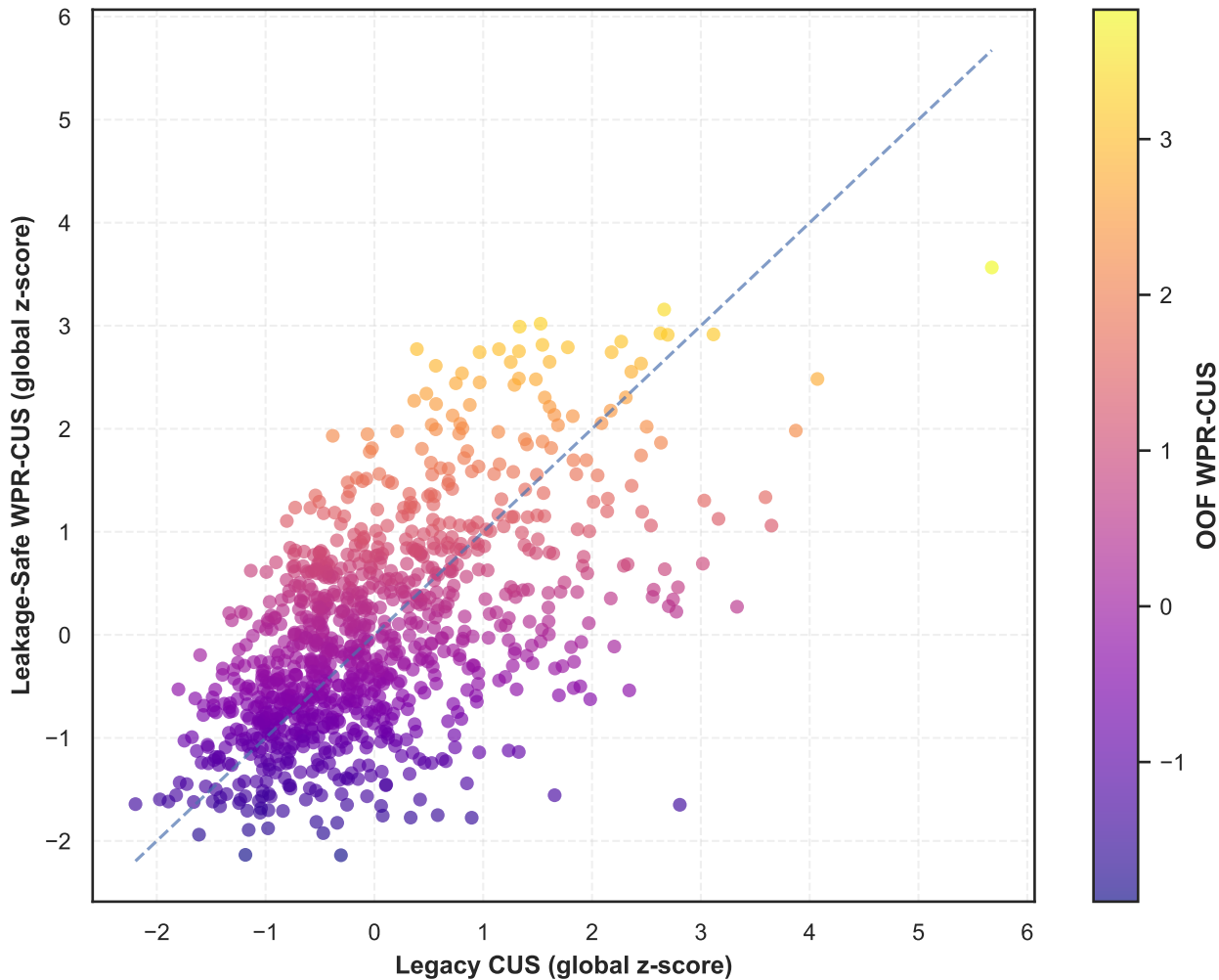
Legacy CUS vs. Leakage-Safe WPR-CUS Spearman rho = 0.555
