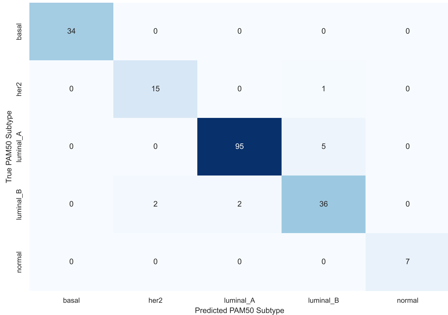
Independent Holdout Confusion Matrix: Logistic Regression
