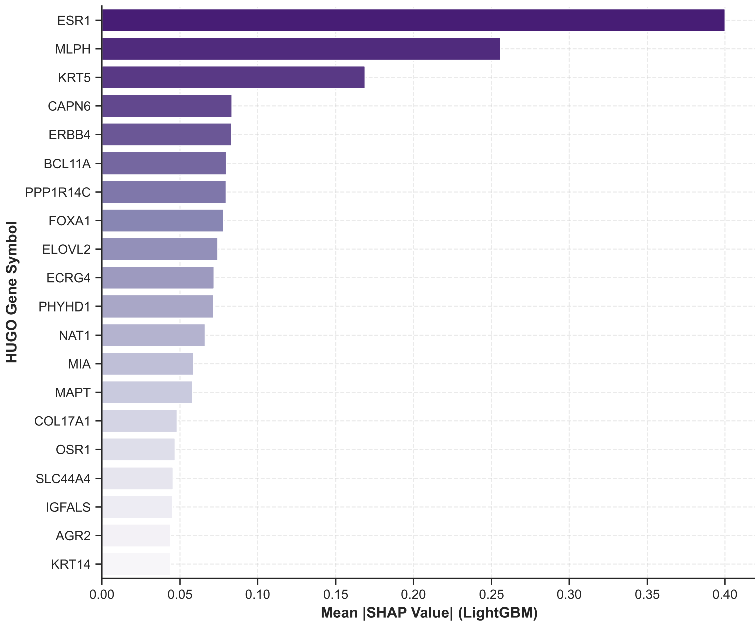
B. Top 20 Non-Linear Model Drivers (Non-Linear Champion)
