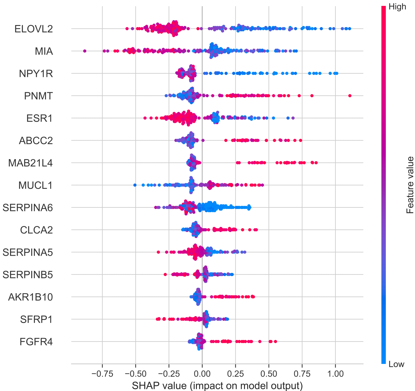
Subtype-Specific SHAP Beeswarm Plot: Her2 (LightGBM)
