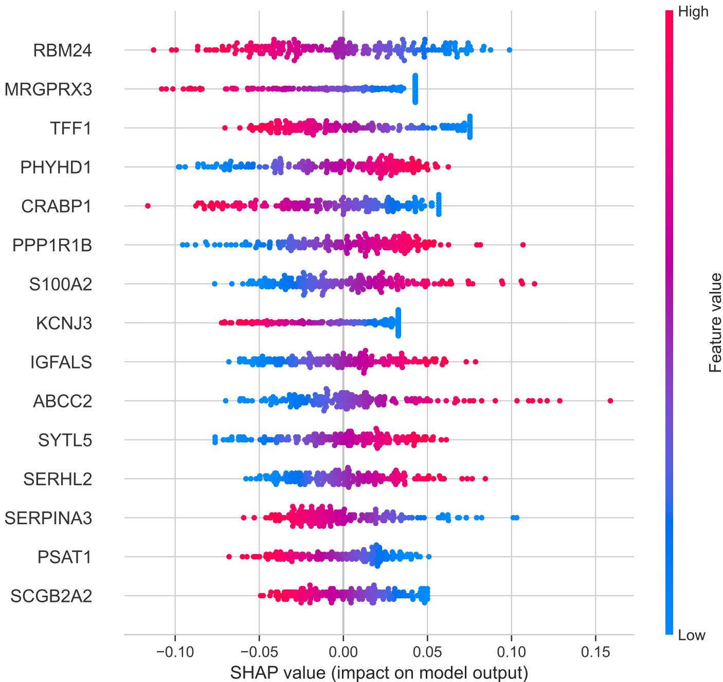
Subtype-Specific SHAP Beeswarm Plot: Luminal A (Linear SVM)
