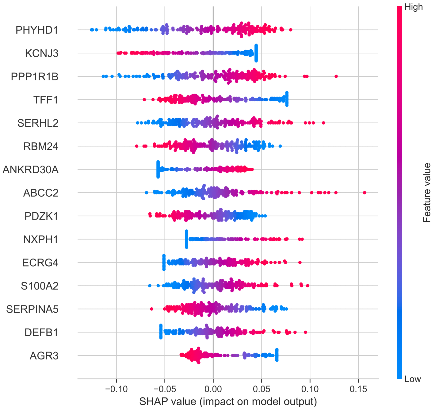
Subtype-Specific SHAP Beeswarm Plot: Luminal B (Linear SVM)
