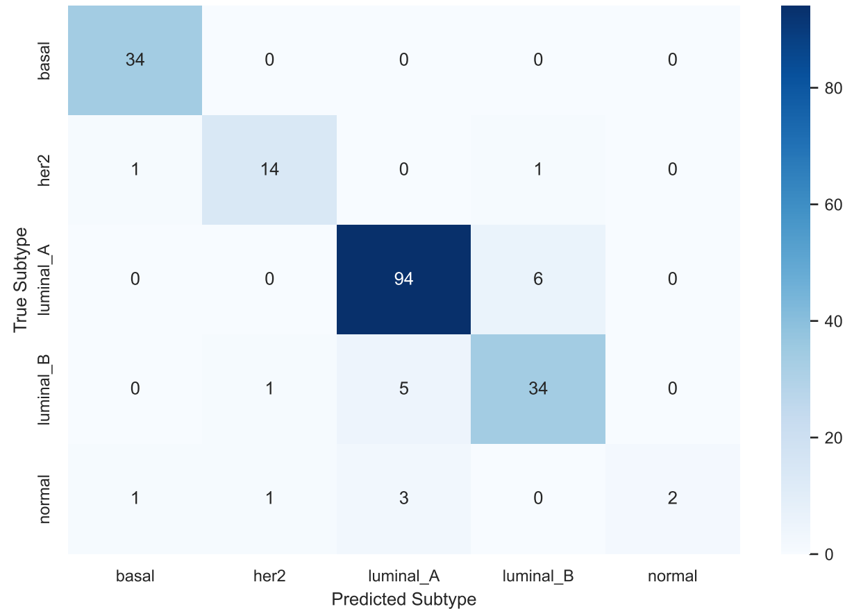
Confusion Matrix: LGBM
