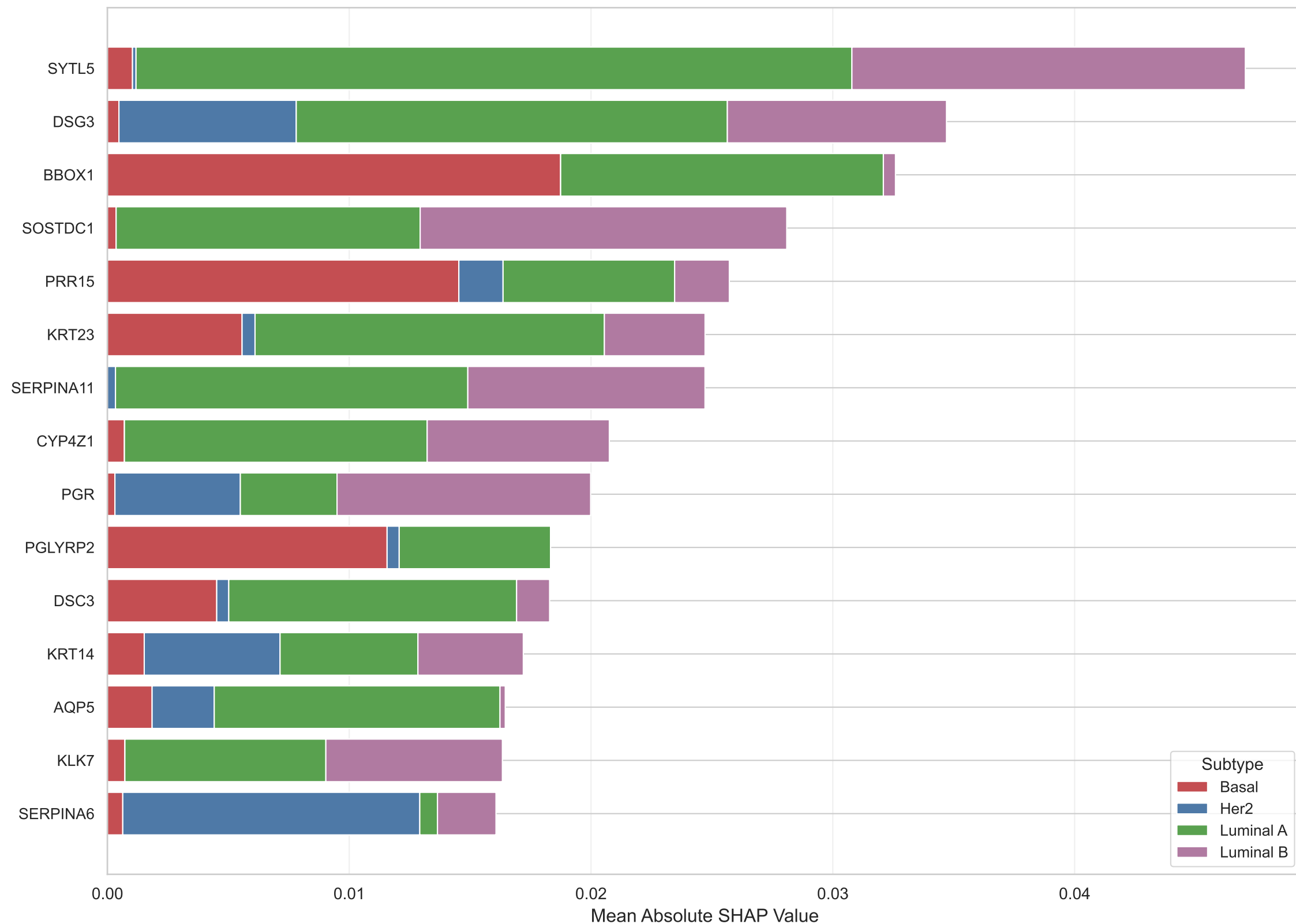
Multi-Class SHAP Impact: Logistic Regression (Linear)
