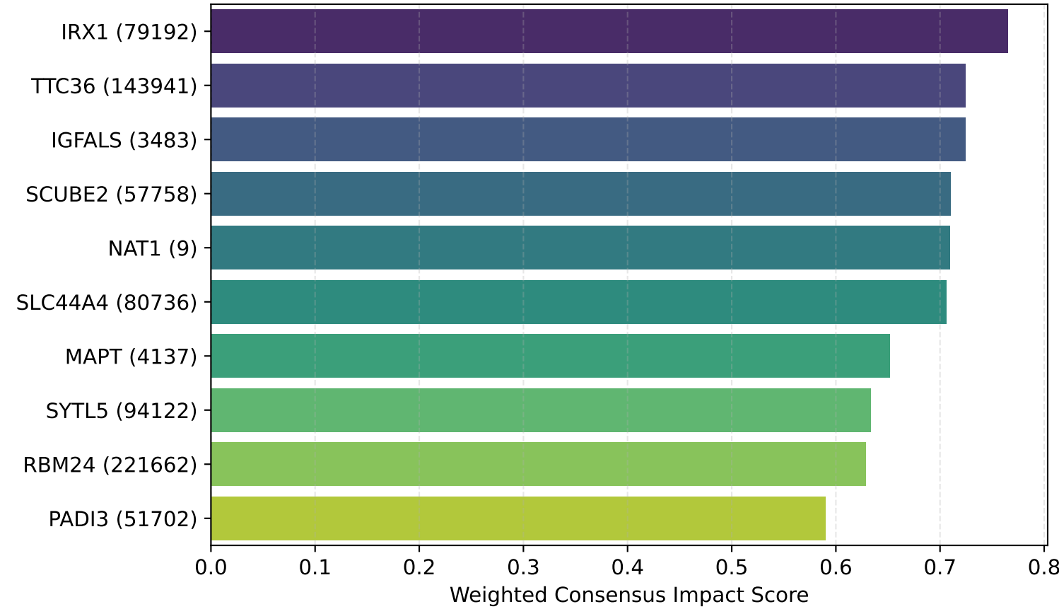
Subtype: NORMAL
