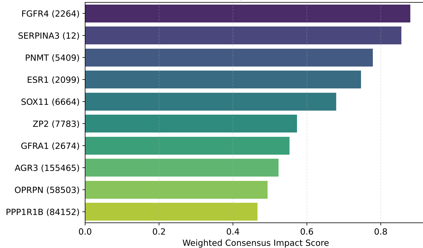
Subtype: LUMINAL_B
