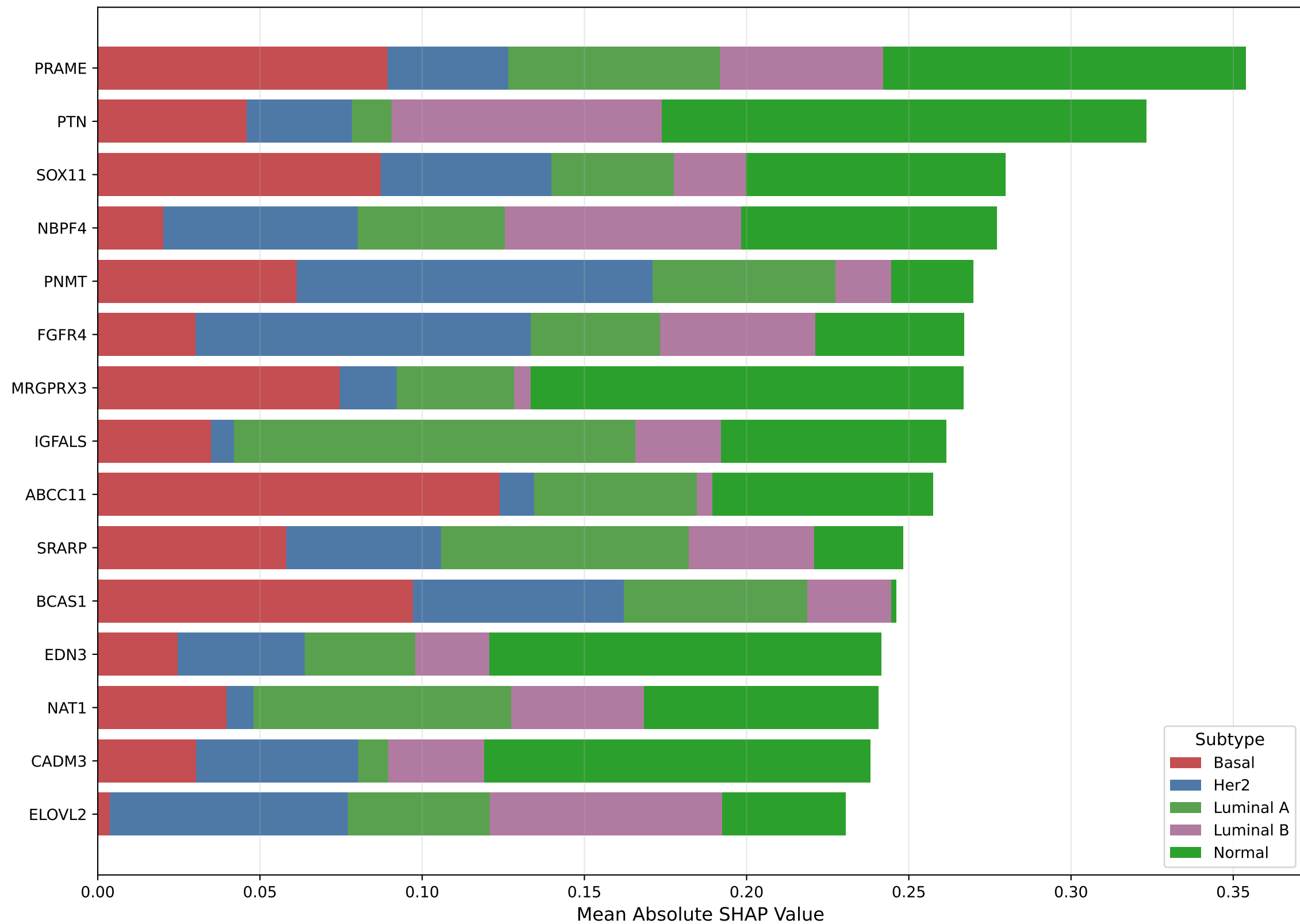
Multi-Class SHAP Impact: Logistic Regression (Linear)
