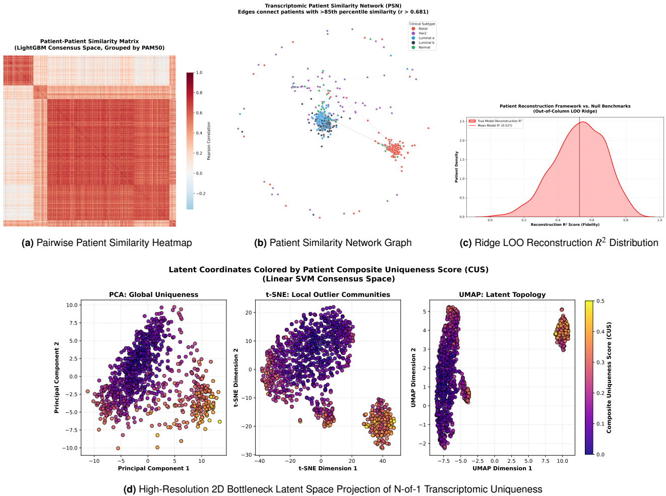
Figure 8. Topological Patient Similarity Networks and Ridge Leave-One-Out Reconstruction Framework.
