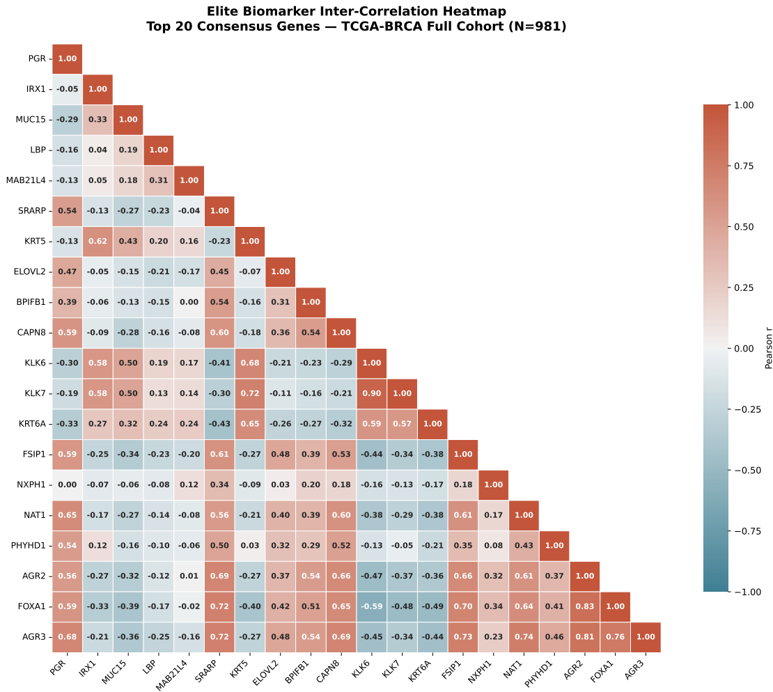
Figure 7. Elite Consensus Biomarker Inter-Correlation Heatmap and Pairwise Co-Expression Matrix.
