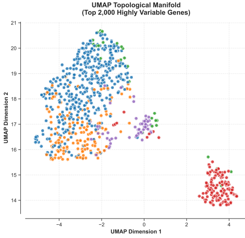
(a) UMAP Topological Manifold (Top 2,000 Genes)
