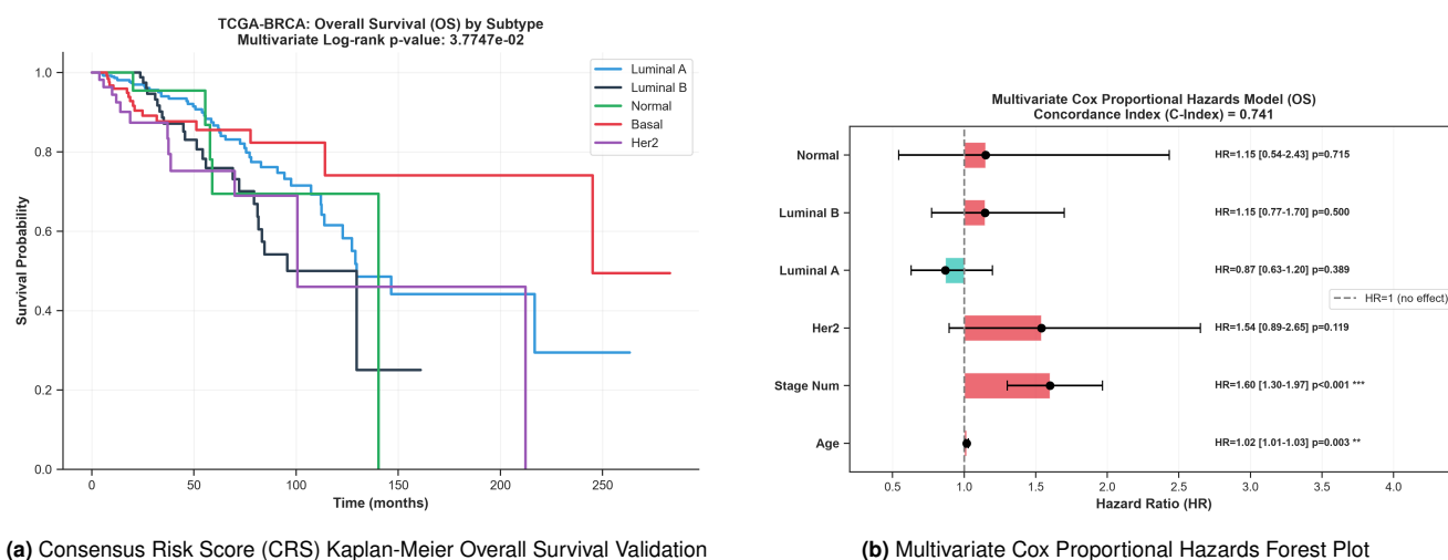
Figure 10. Consensus Risk Score (CRS) Prognostic Overall Survival Stratification and Cox Hazard Ratios.
