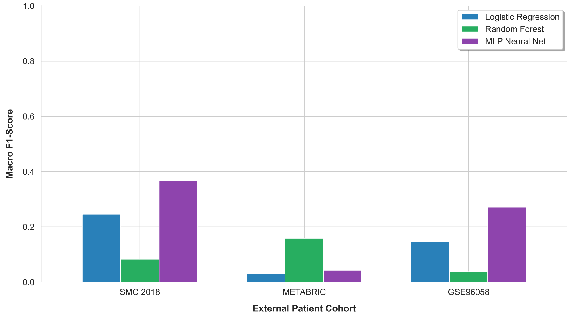
Cross-Platform External Validation Performance (Macro F1-Score)
