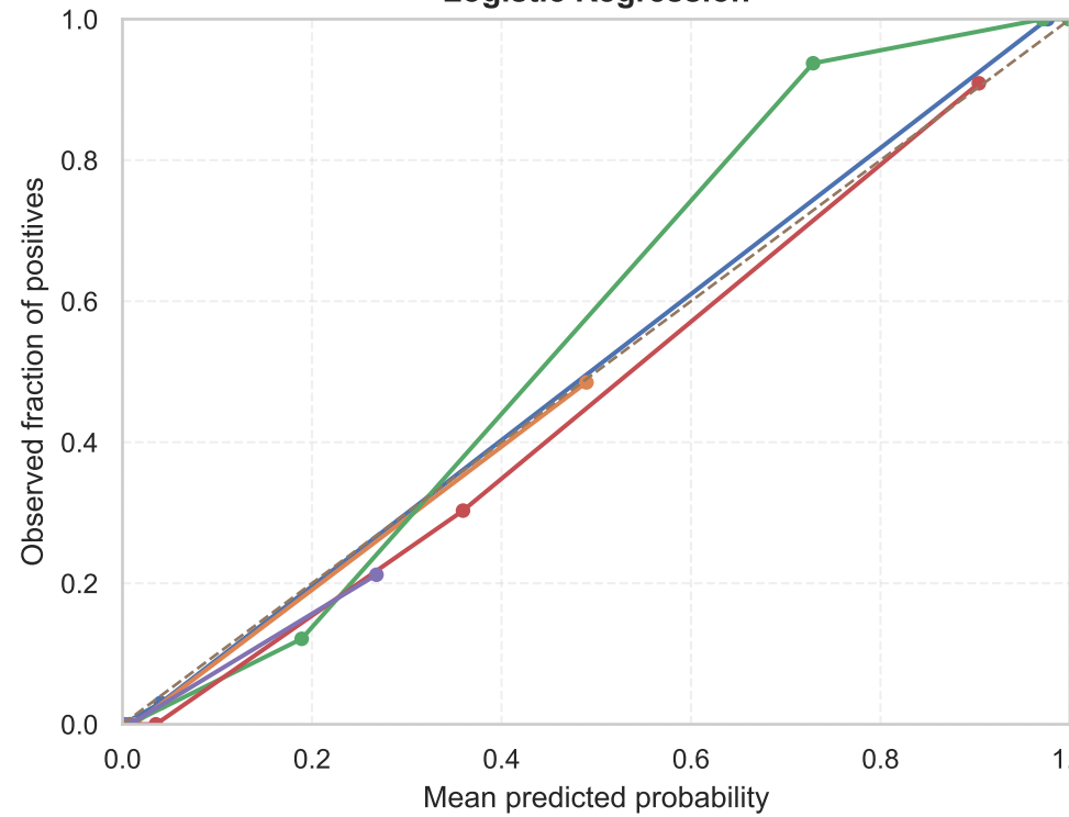
Logistic Regression
