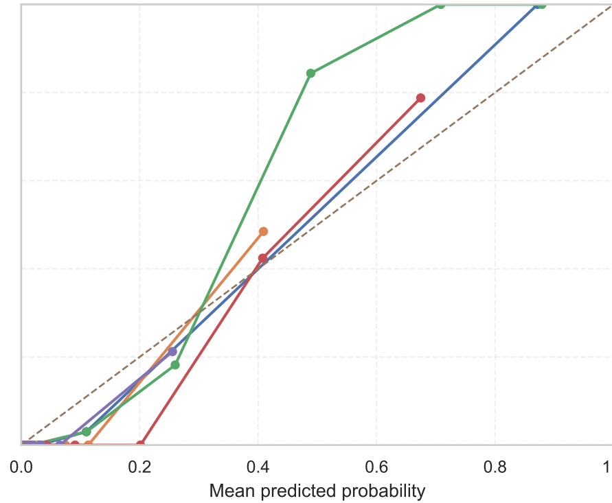
Random Forest
