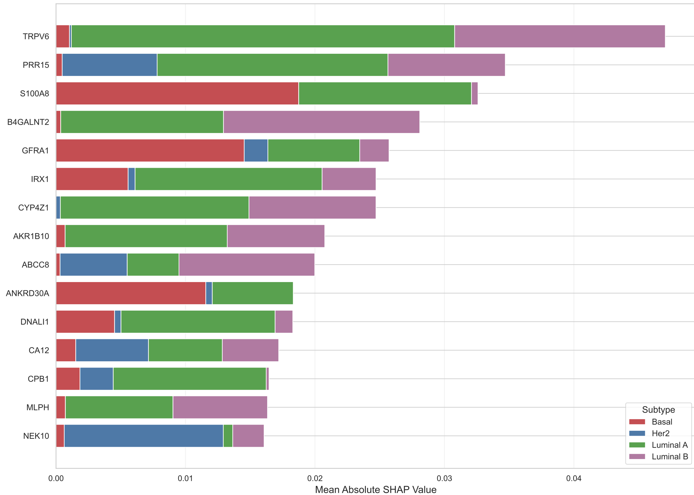
Multi-Class SHAP Impact: Logistic Regression (Linear)
