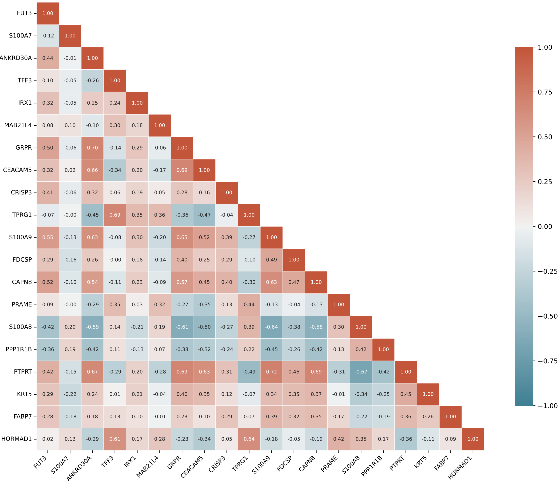
Elite Biomarker Inter-Correlation Heatmap Top 20 Consensus Genes — TCGA-BRCA Full Cohort (N=945)
