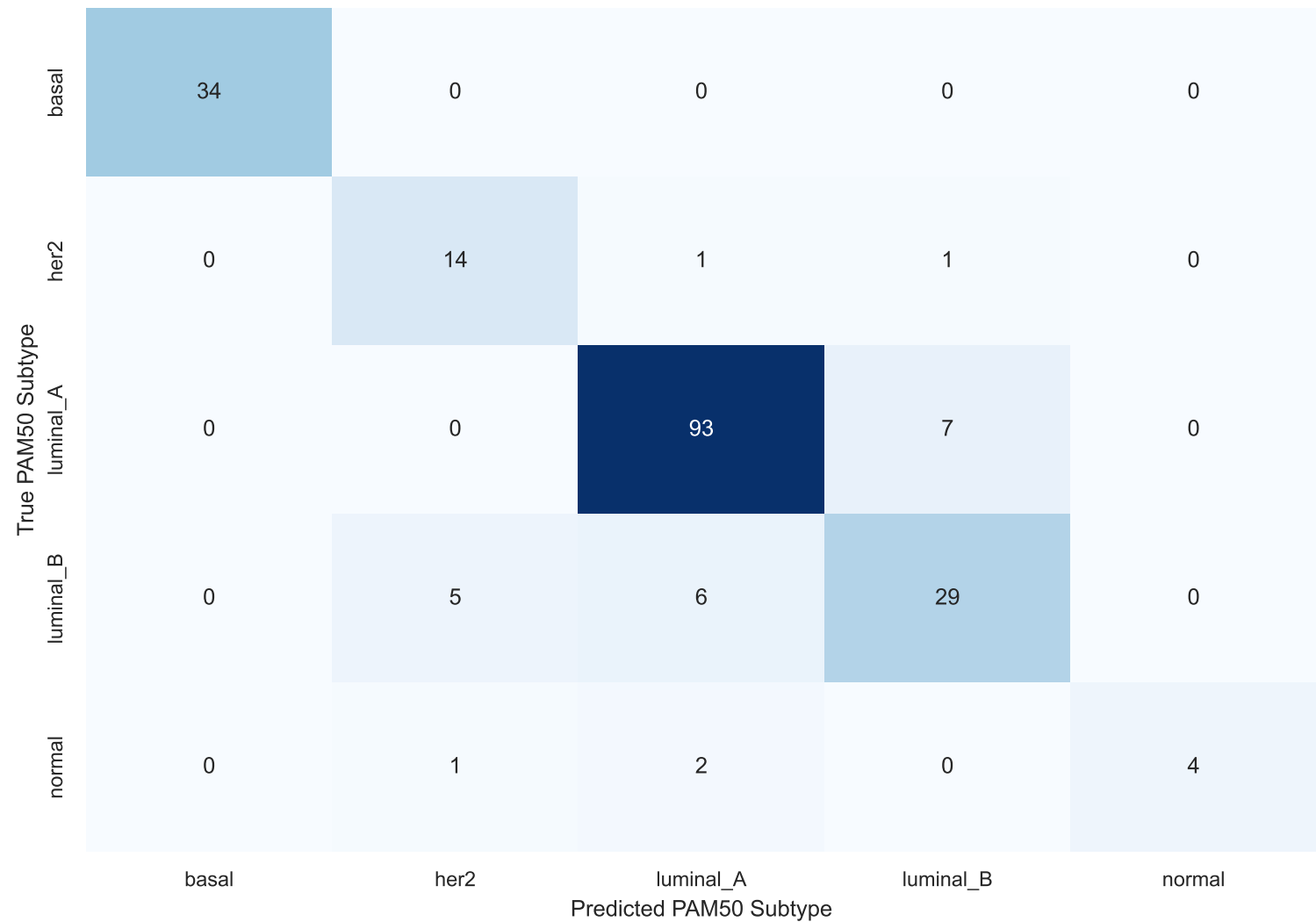
Independent Holdout Confusion Matrix: MLP
