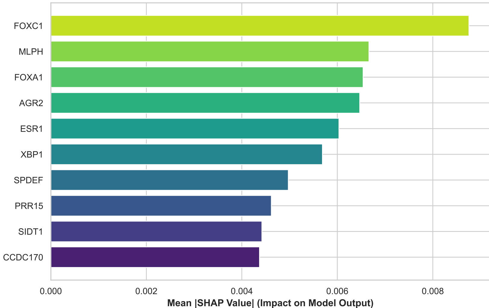
Subtype: BASAL Random Forest SHAP Feature Importance
