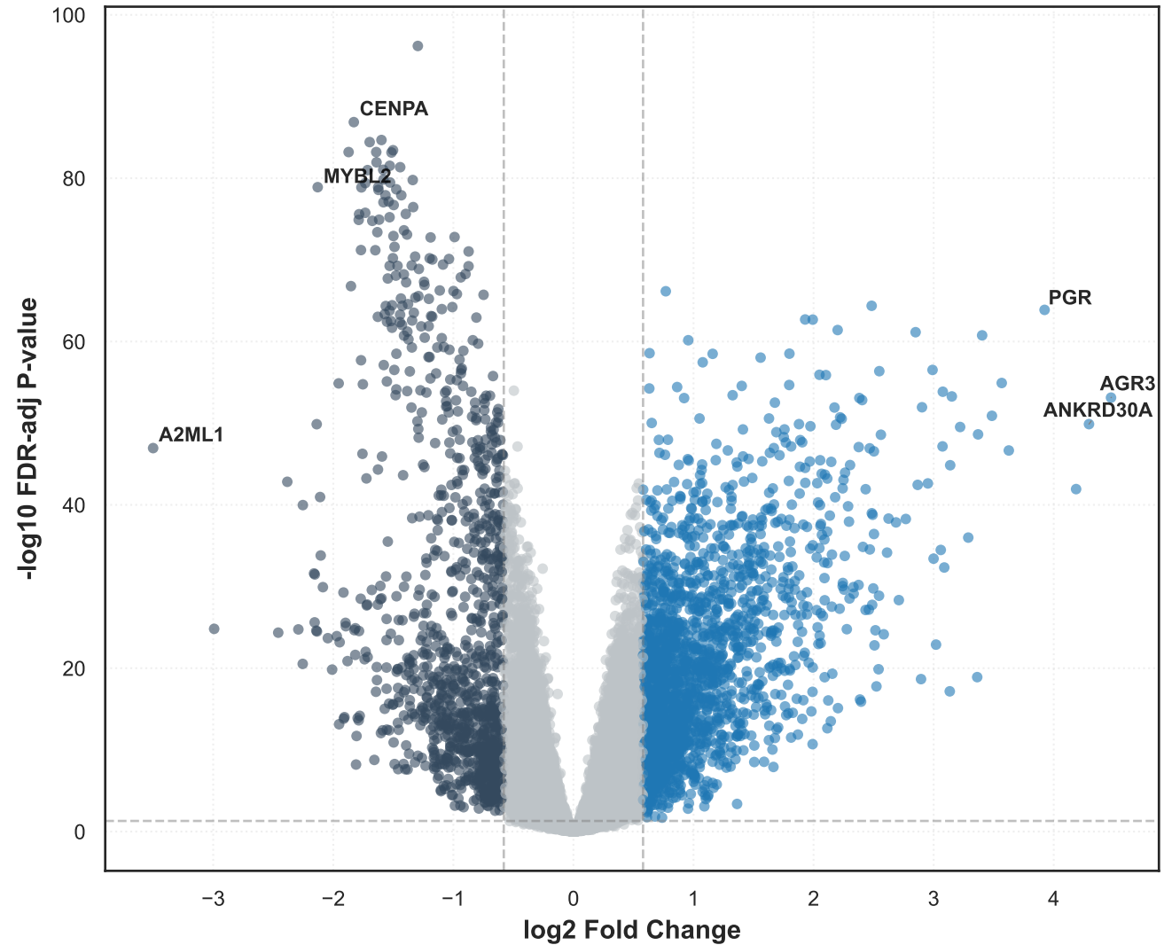
DGE Volcano Plot: Luminal A One-vs-Rest Welch's t-test (FDR < 0.05, |LFC| > 0.58)
