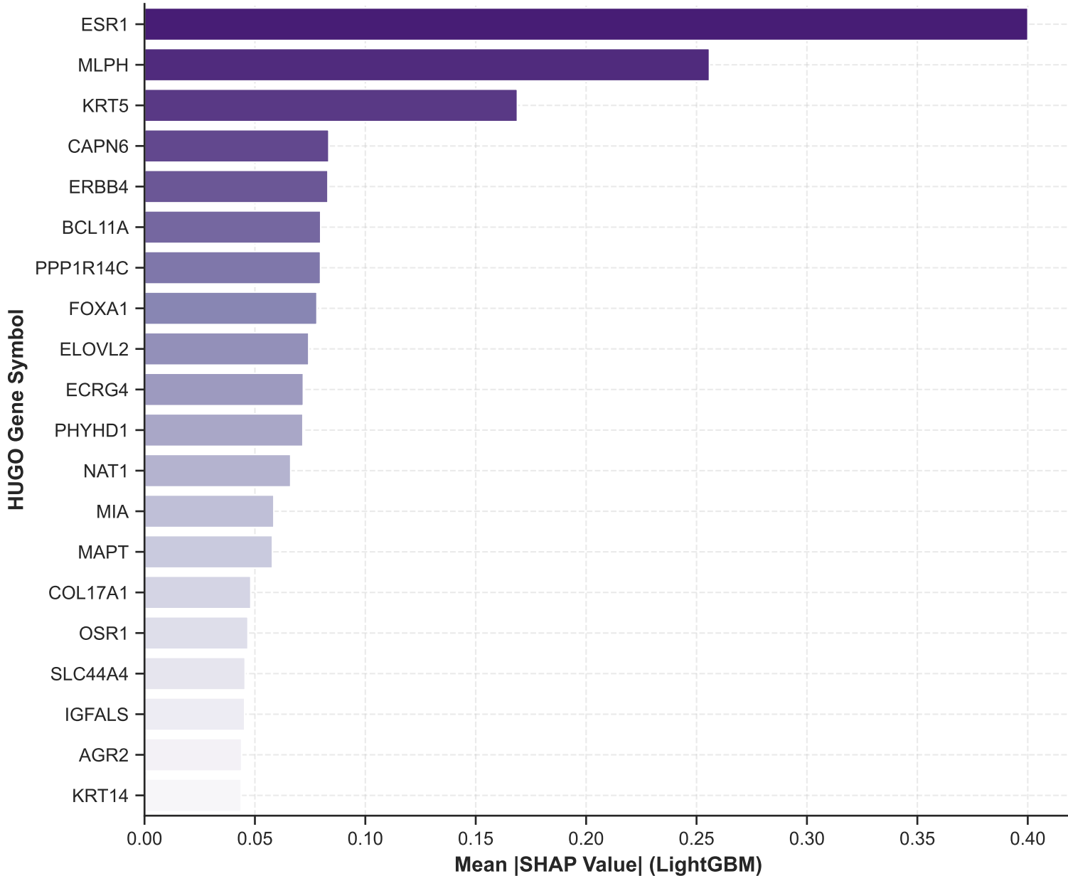
B. Top 20 Non-Linear Model Drivers (LightGBM (Non-Linear))
