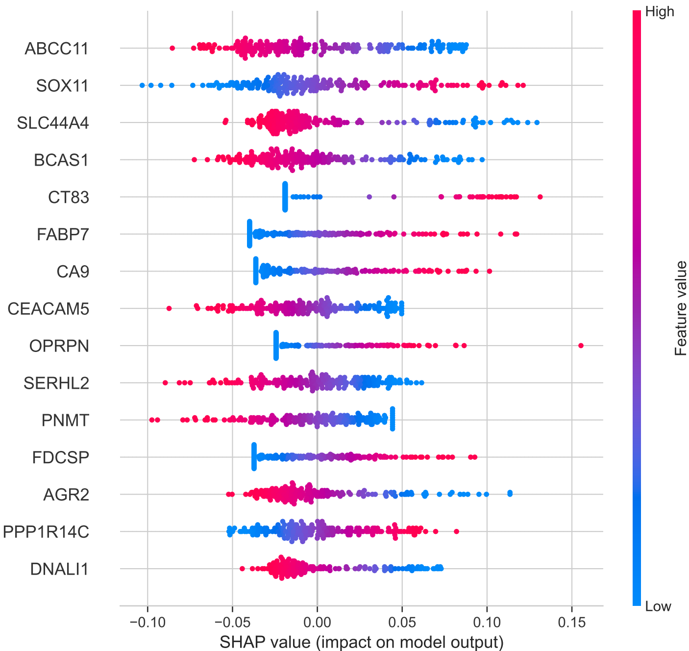
Subtype-Specific SHAP Beeswarm Plot: Basal (Linear SVM)
