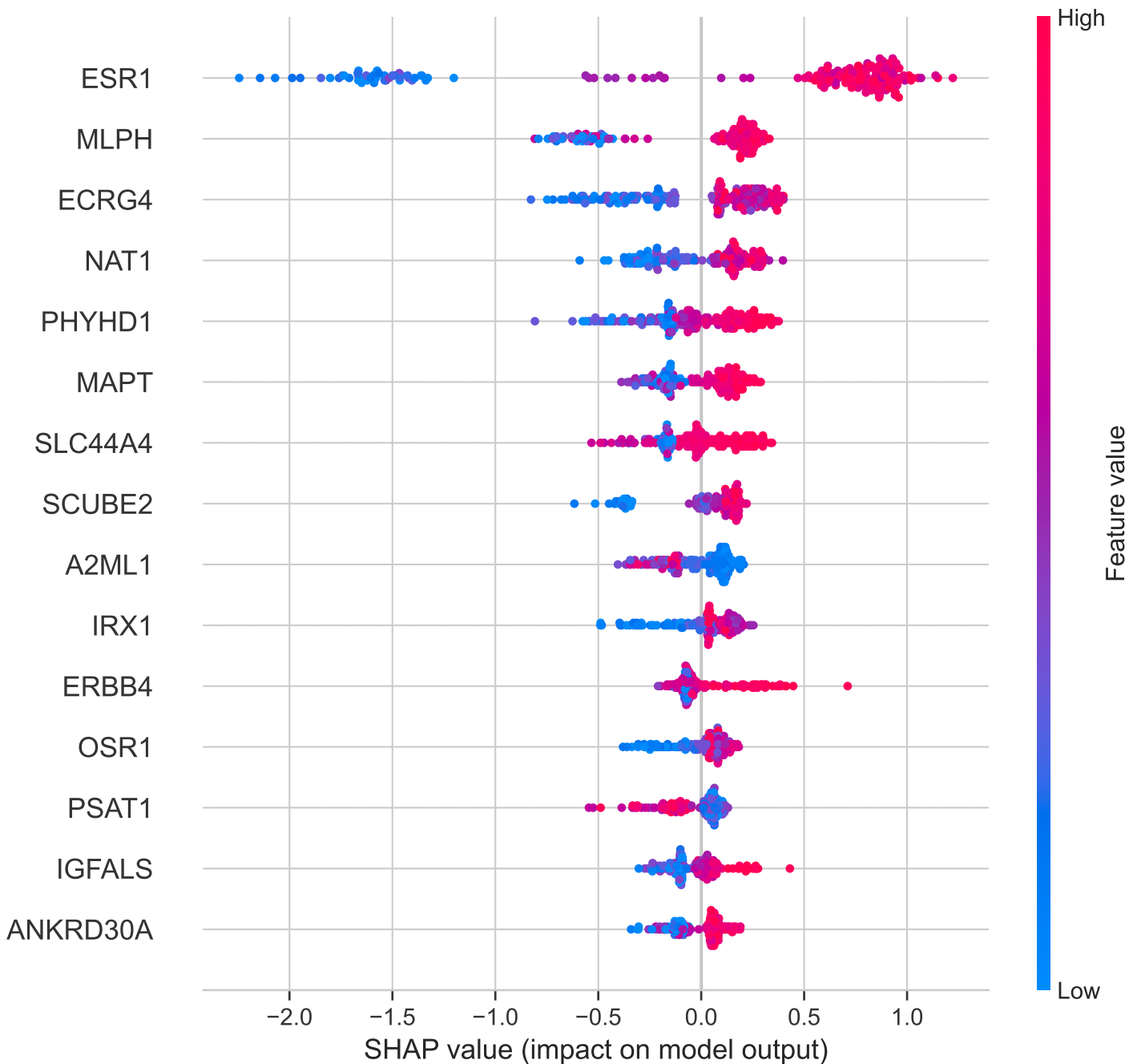
Subtype-Specific SHAP Beeswarm Plot: Luminal A (LightGBM)
