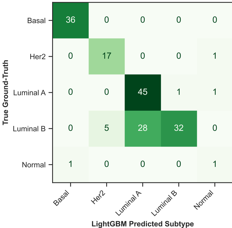
Confusion Matrix: SMC 2018 (LightGBM Transfer) Macro F1: 0.728
