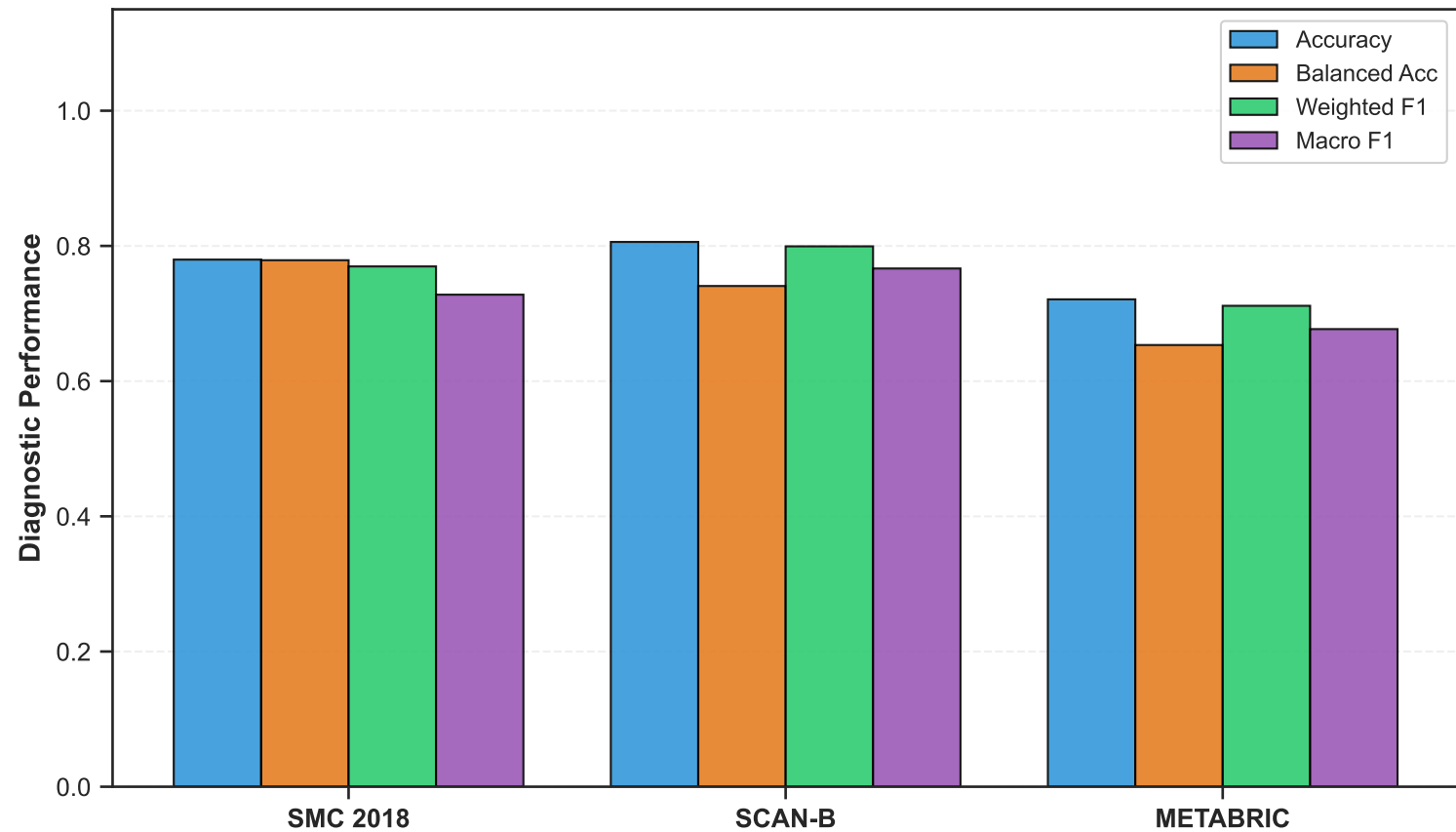
Cross-Platform Validation: Non-Linear Classifier (LightGBM)
