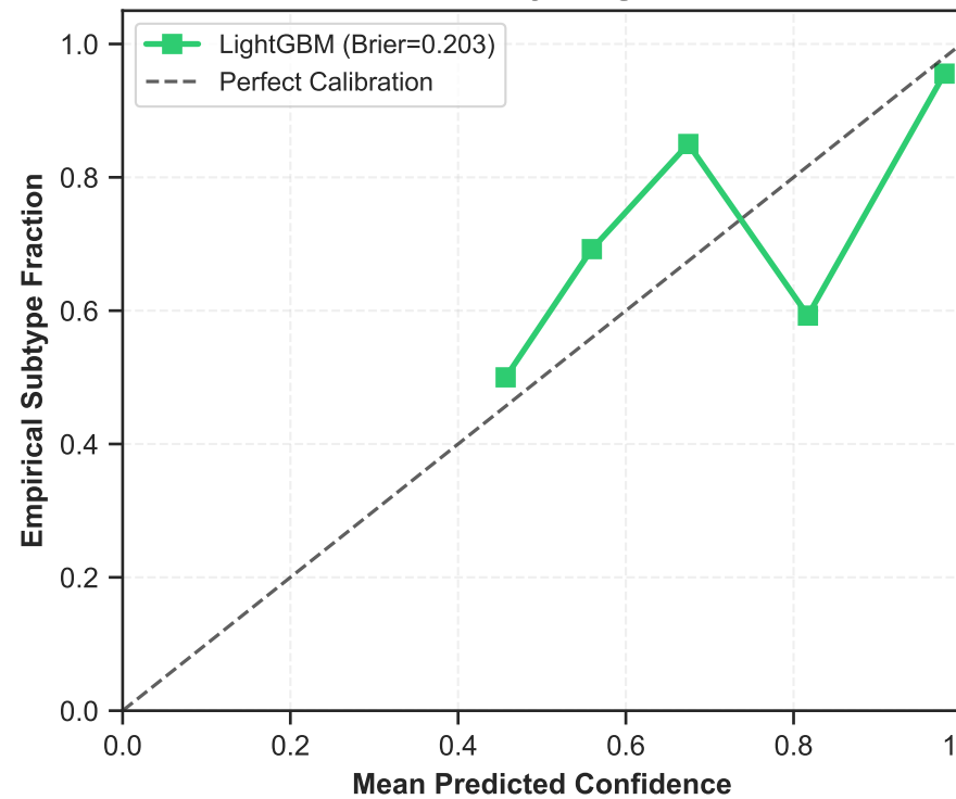
TCGA Holdout Reliability Diagram
