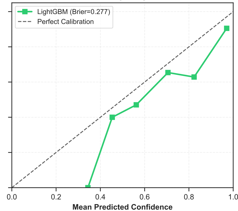
SCAN-B Reliability Diagram
