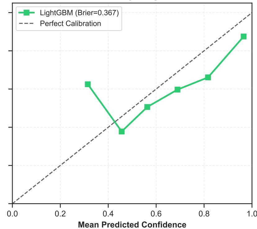
METABRIC Reliability Diagram
