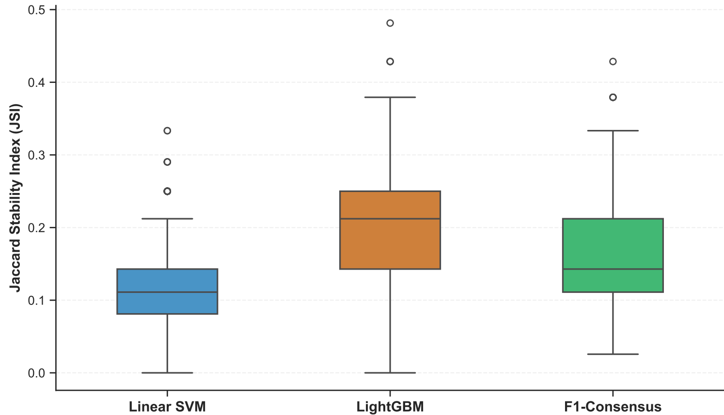
Bootstrap Feature Selection Stability (B=50 Resamples)
