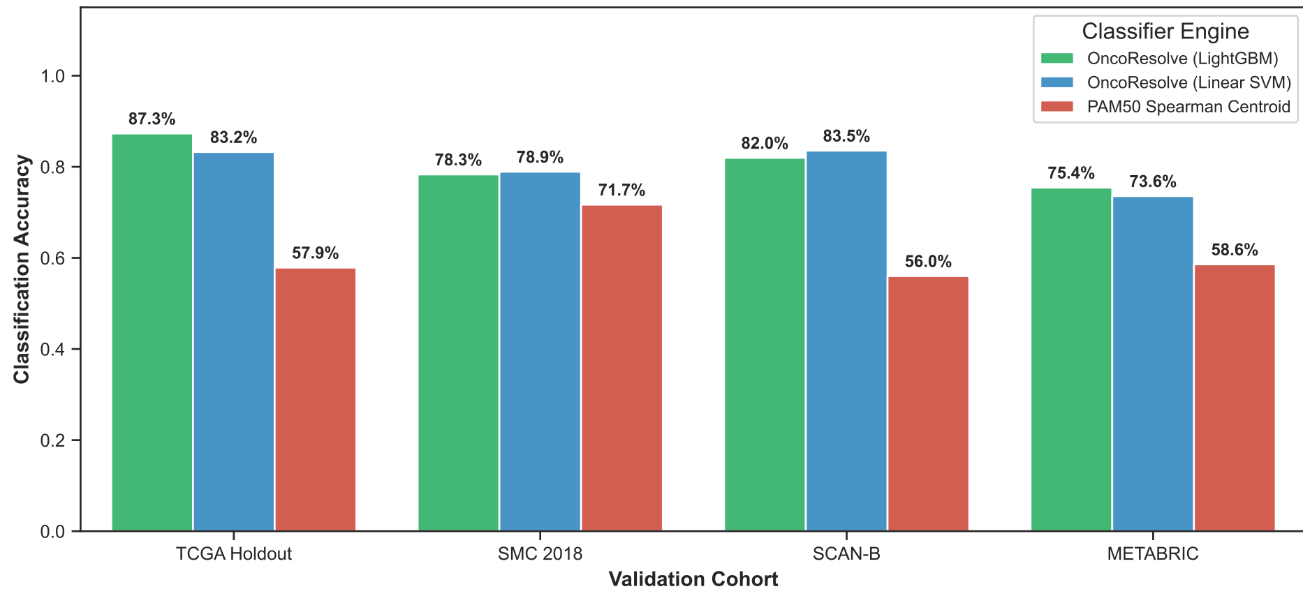
Comparative Subtyping Performance: OncoResolve vs. PAM50 Spearman Centroid
