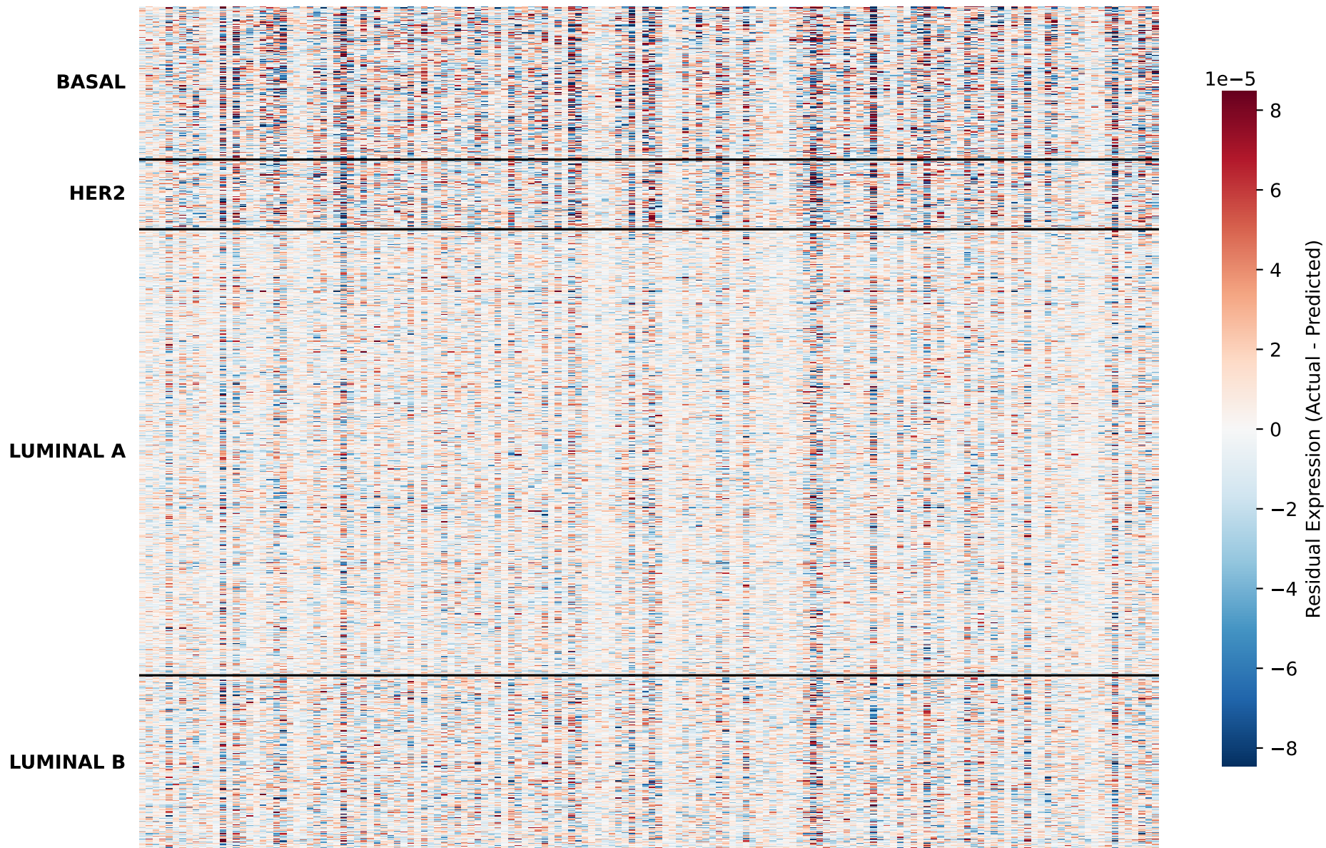
Transcriptomic Uniqueness Residuals Heatmap (Dual-Architecture Consensus Space)
