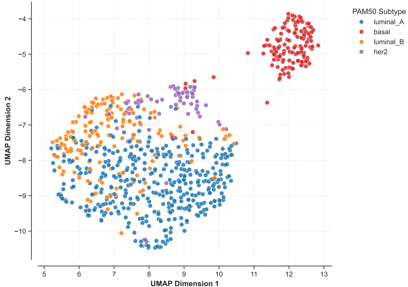
UMAP Topological Manifold (Top 5,000 Highly Variable Genes)
