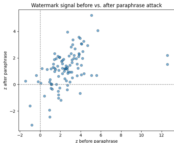
Figure 3: Watermark signal before vs after paraphrase attack
