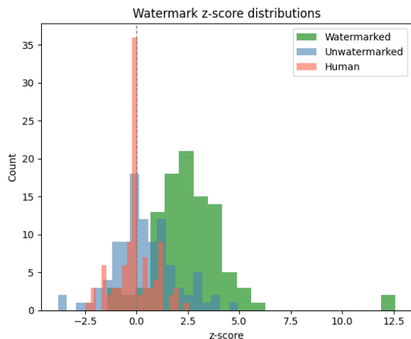
Figure 2: Watermark z-score distributions
