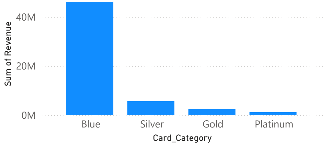
Sum of Revenue by Card_Category
