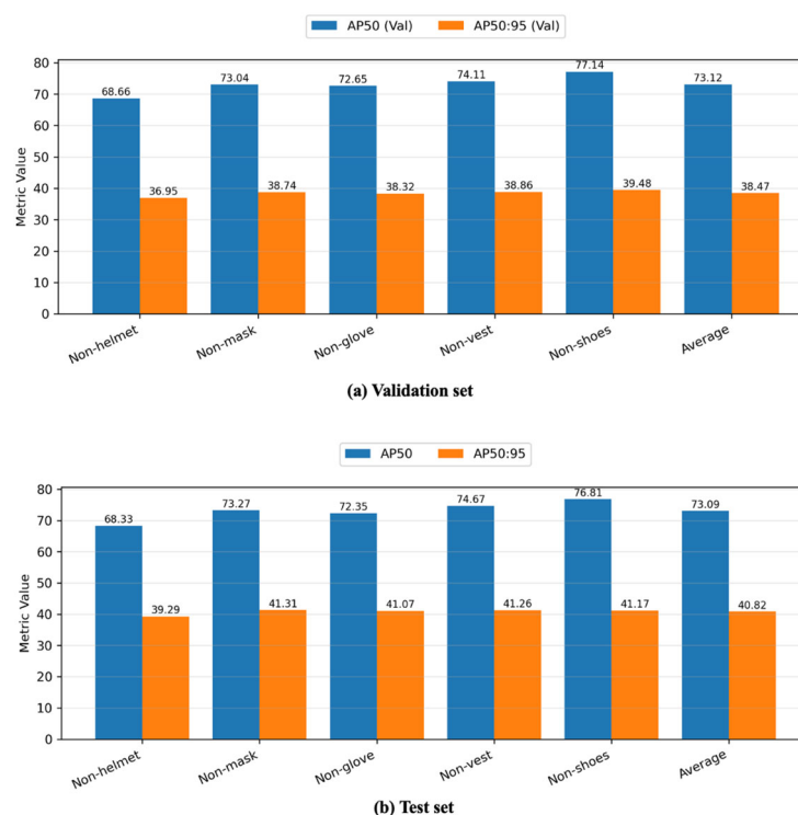
Figure 11. Class-wise performance on validation and test set.
