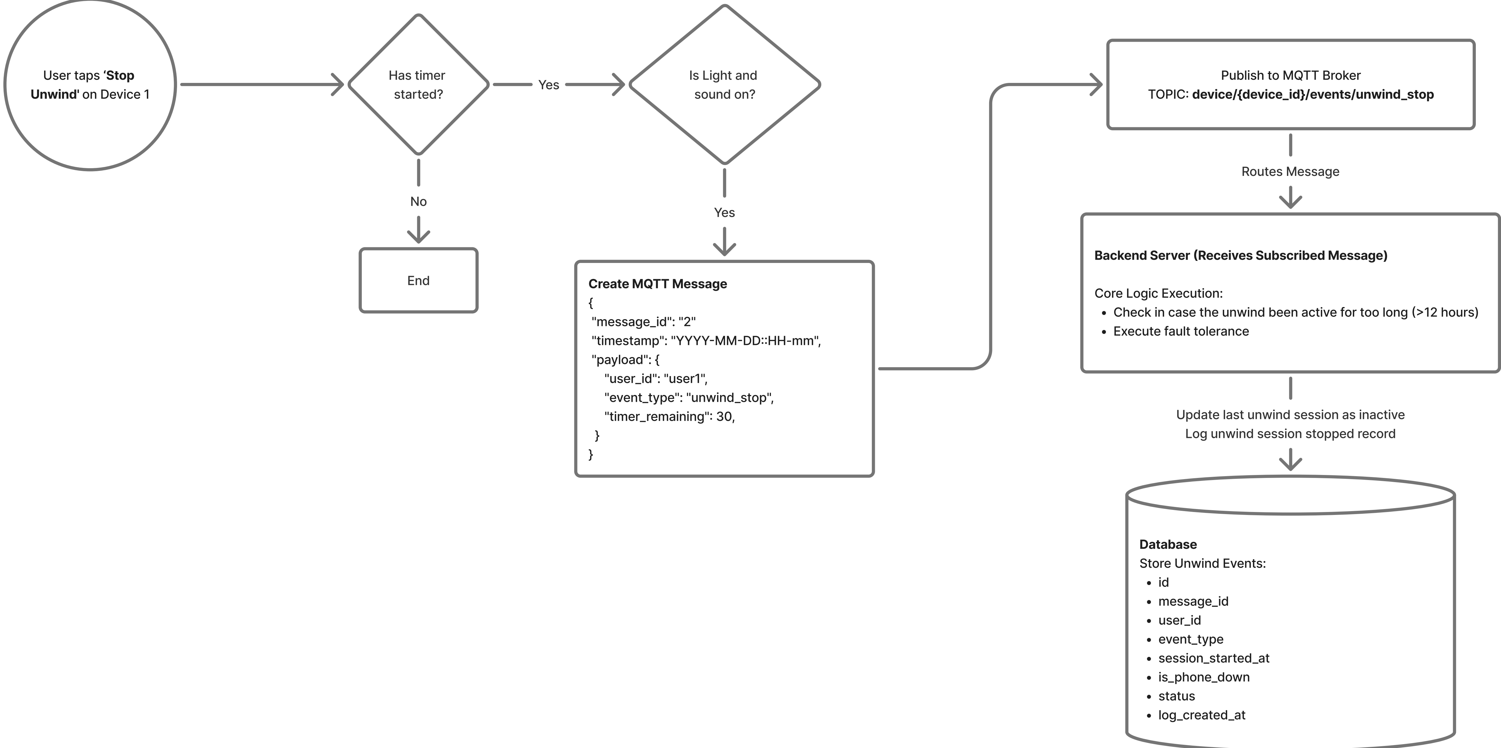
Data Flow - Unwind Session Stop
