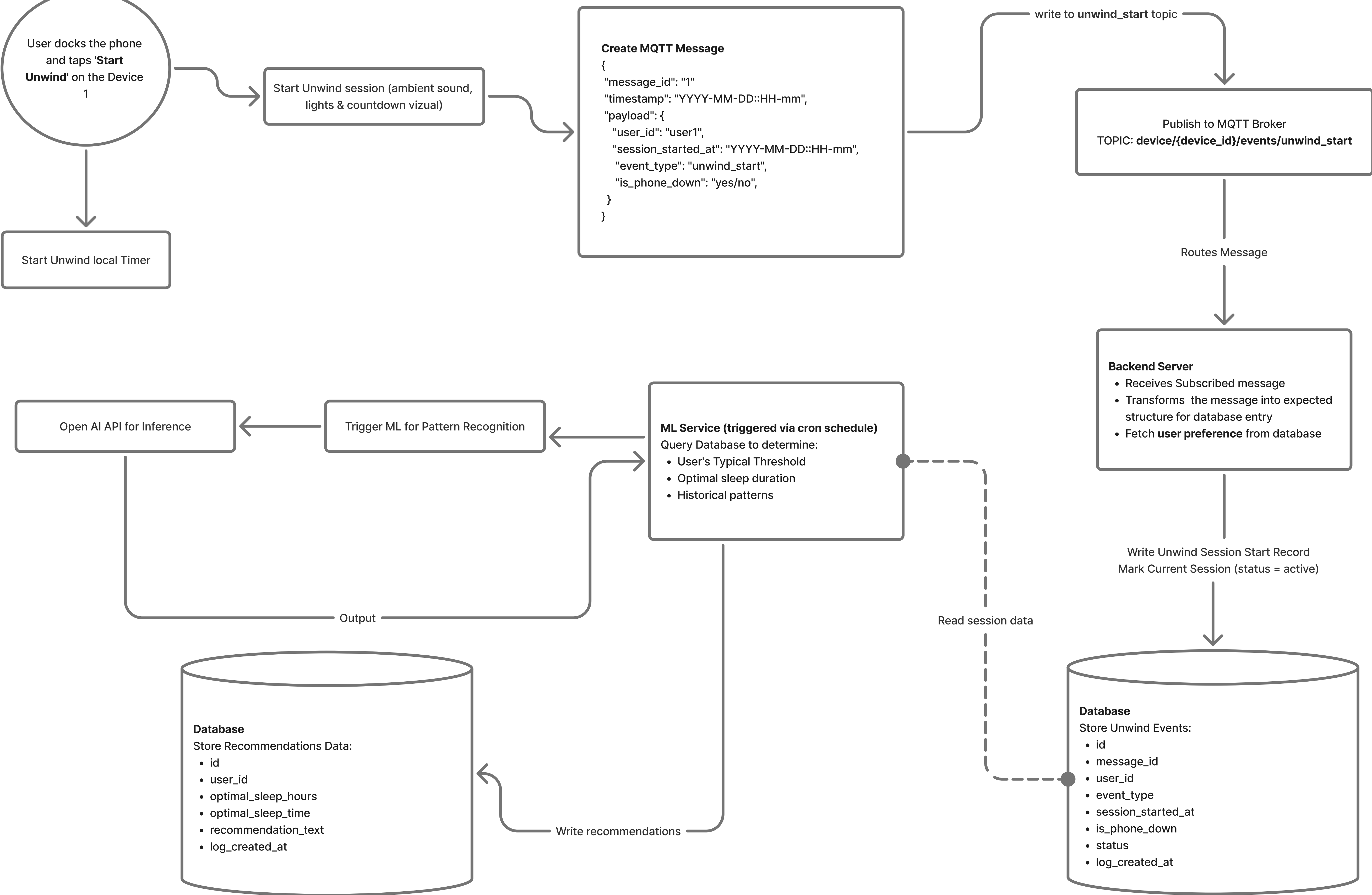
Data Flow - Unwind Session Start
