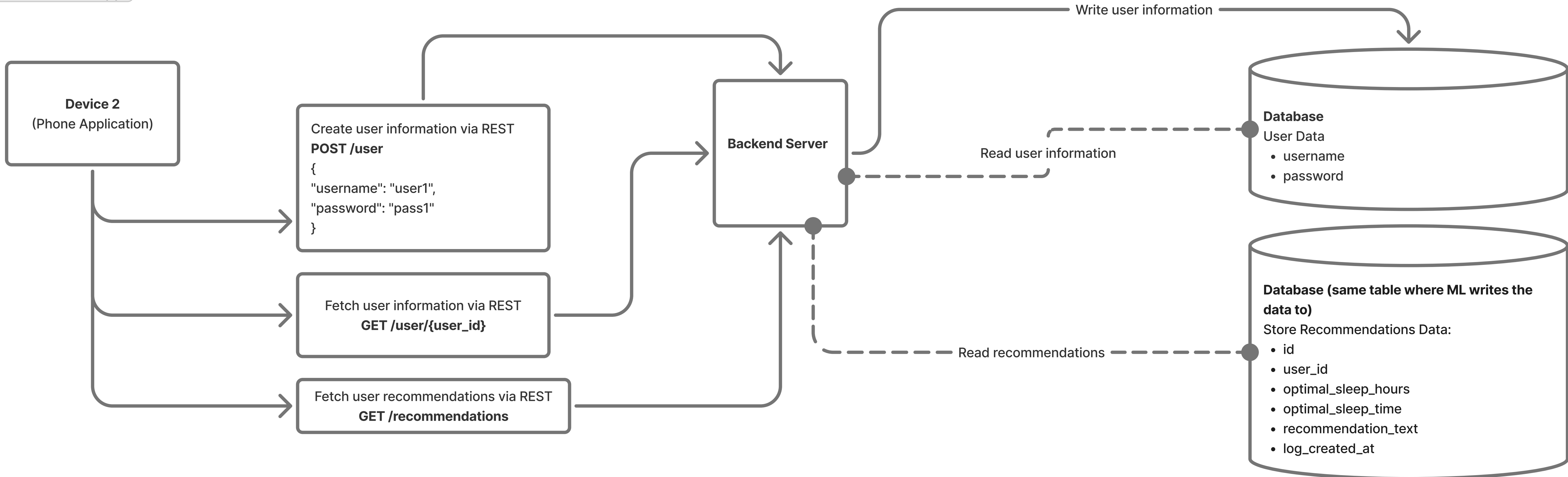
Data Flow - Phone App
