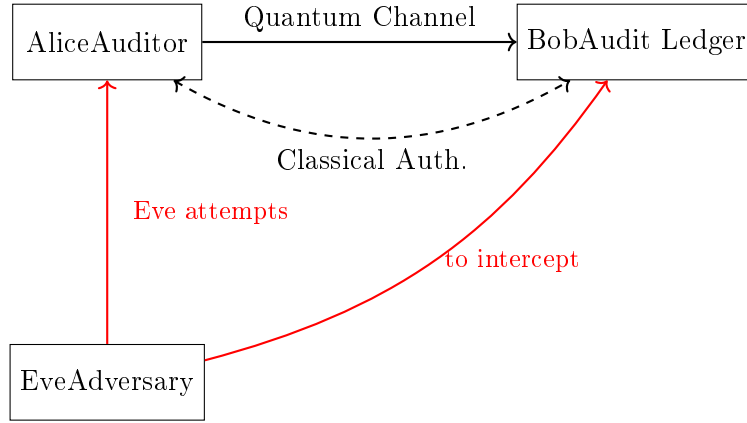
Figure 1: BB84 setup for SCX audit. Alice (auditor) sends M_t encoded as polarized photons. Eve (adversary) may attempt to eavesdrop on the quantum channel. The classic
