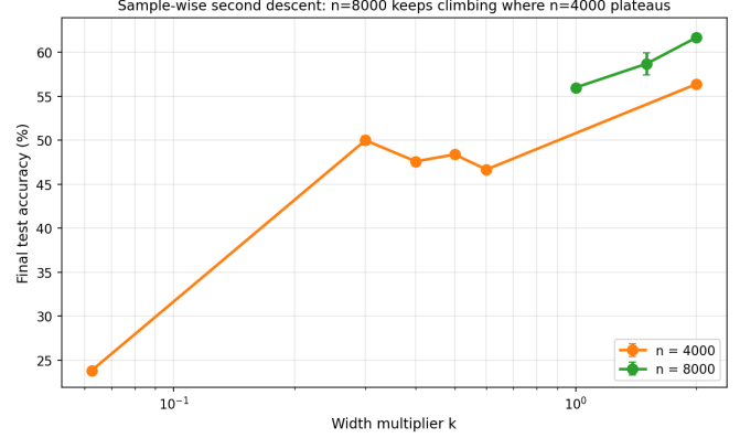
(b) Final-epoch n -slice audit of the same sweep.
