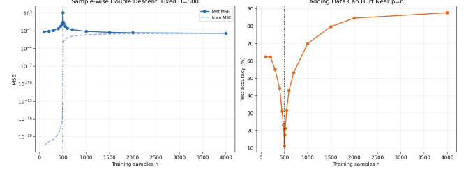
(b) Sample-wise: test MSE vs. n for fixed p = 500 .
