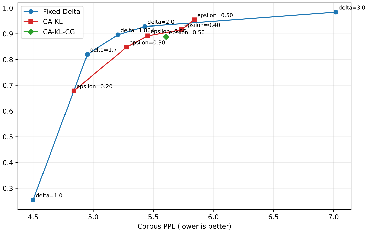
Standard KGW detection rate
