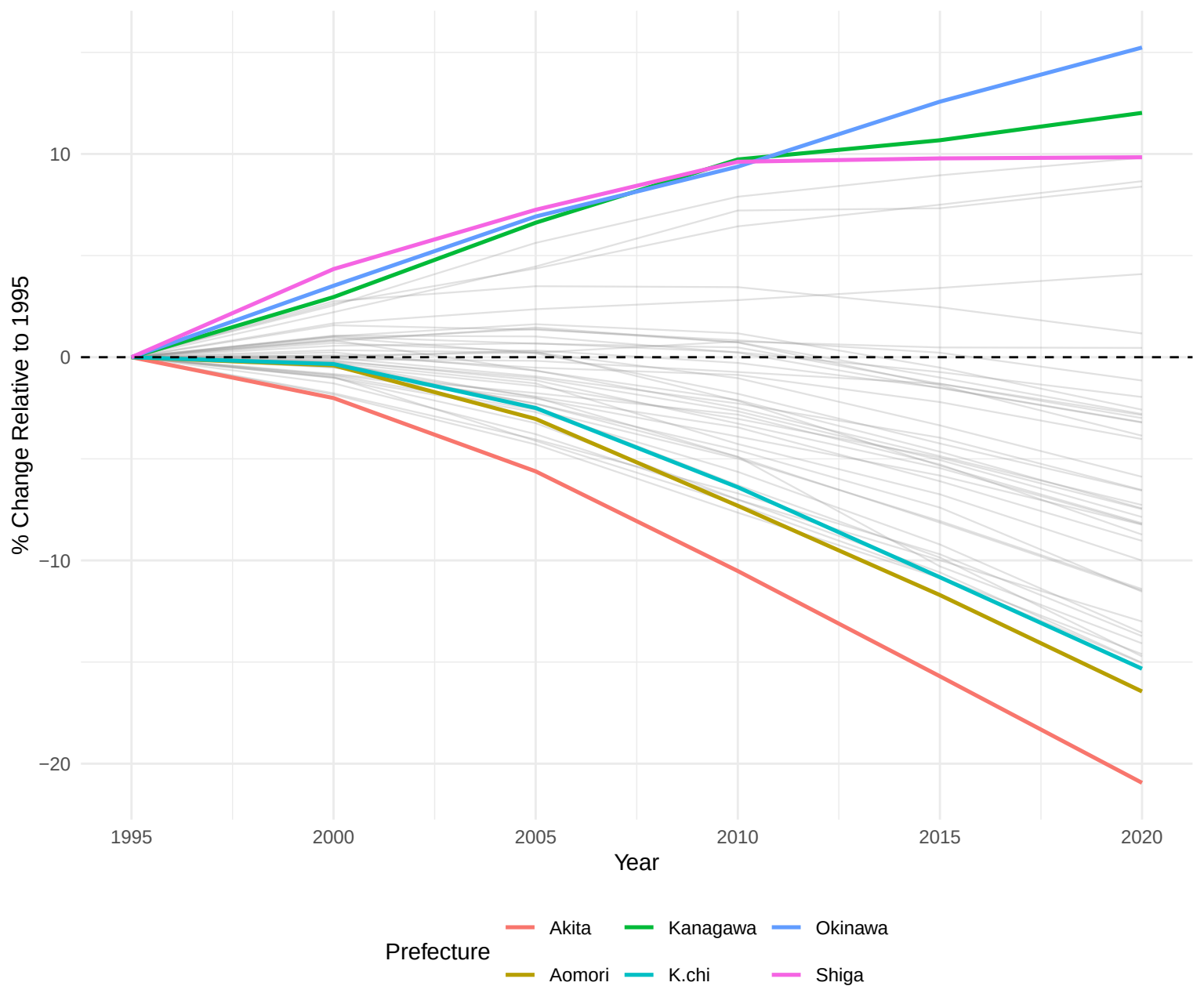
Population Change by Prefecture (1995--2020)
