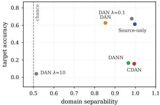
(b) Separability does not predict transfer
