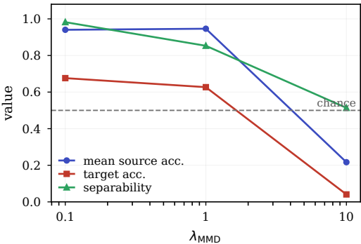
(a) DAN alignment-strength sweep
