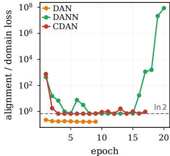
(b) Alignment loss
