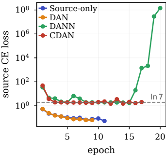
(a) Classification loss
