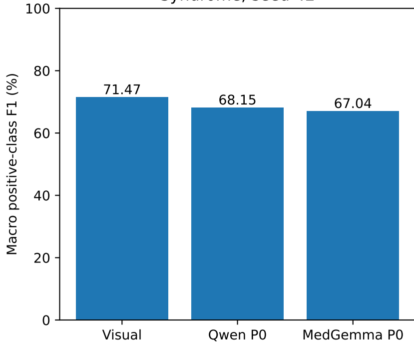
Syndrome; seed 42
