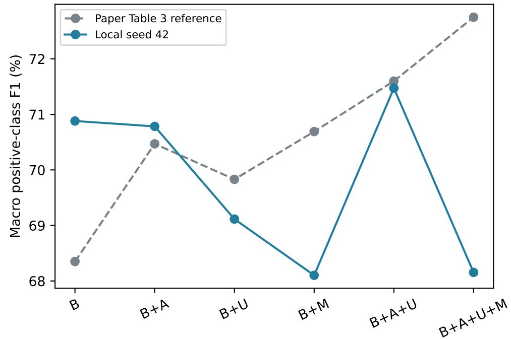
Syndrome
