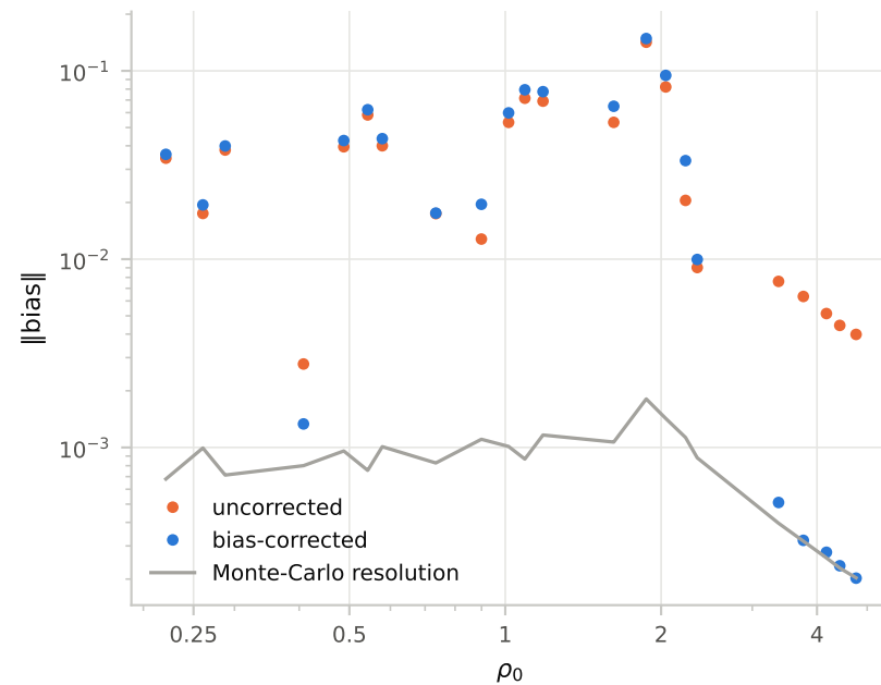
(b) adaptive gate: bias vs its clean-data target
