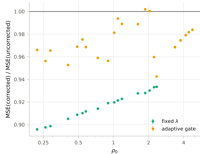
(c) value of the correction vs own target
