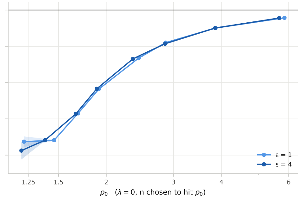
(b) no ridge (plain OLS); gate \hat{\rho} \geq 1
