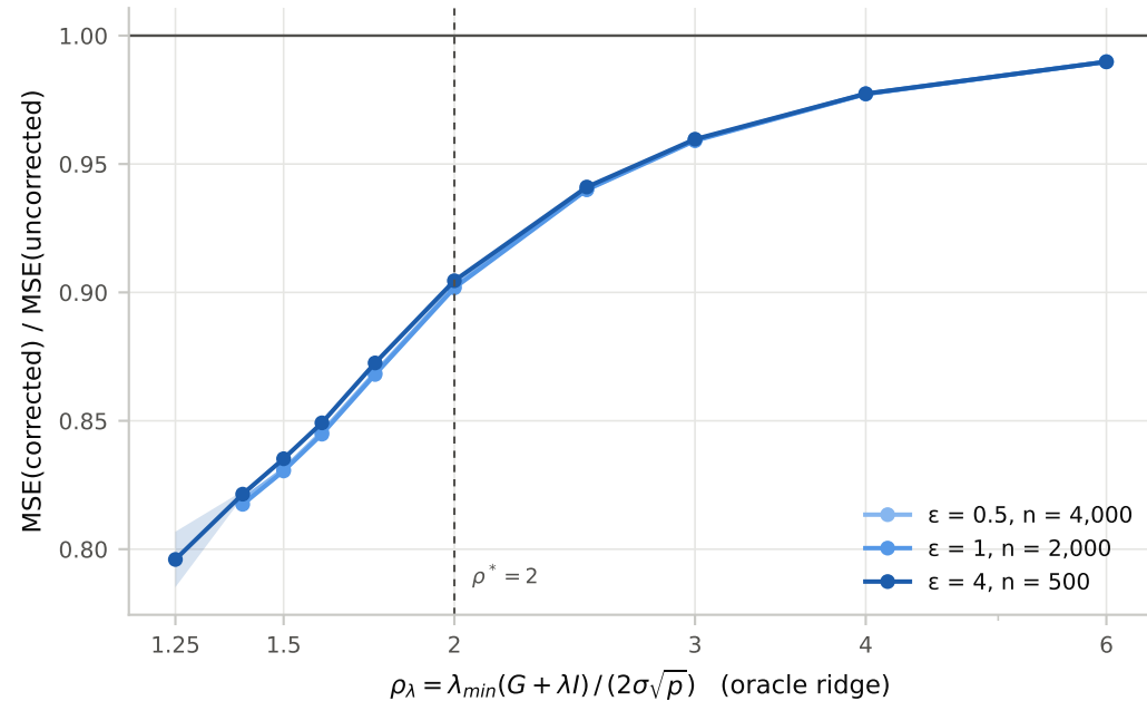
(a) ridge regime, \lambda set to hit \rho_\lambda ; gate \hat{\rho} \geq 1
