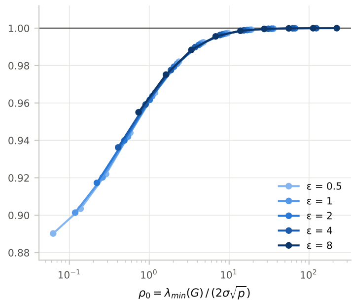
(c) vs \hat{\beta}_\lambda , \ell = 0 (ridge always on)
