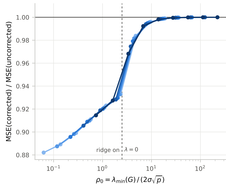
(a) vs protocol target \hat{\beta}_\lambda ( \ell = 0.8\lambda_{\min} )
