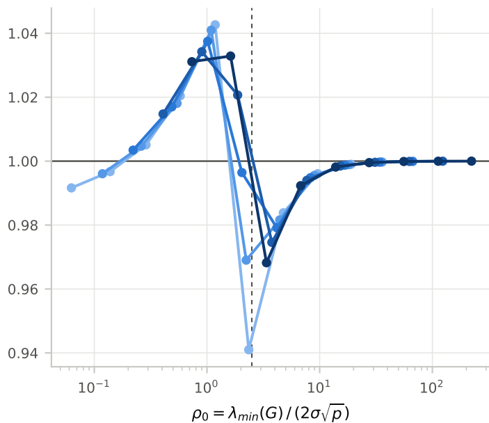
(b) vs sample OLS \hat{\beta} ( \ell = 0.8\lambda_{\min} )
