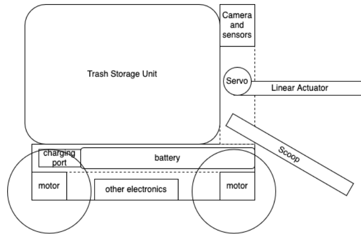
FIGURE 4.3.2.1: COMPONENTS LAYOUT
