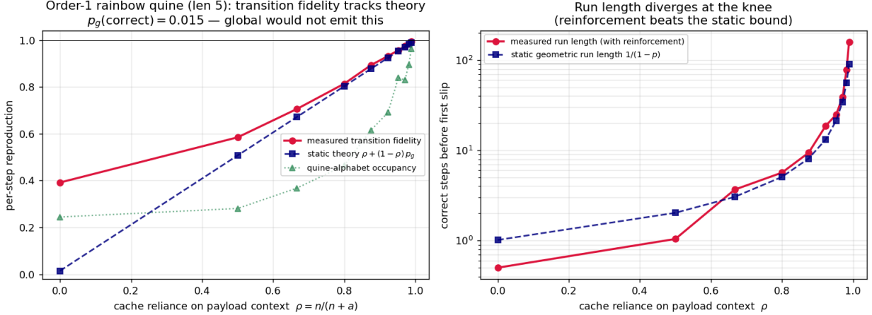
Figure 1: Order-1 rainbow quine over the rarest symbols ( p_g = 0.015 ). Left : measured transition fidelity tracks the closed form (??); alphabet occupancy lags but \rightarrow 0.96 (the walk re-enters after a slip). Right : measured run length beats the static geometric bound 1/(1 - p_{\text{step}}) once past the knee—self-reinforcement. Reproduced by demo_contagion.py .
