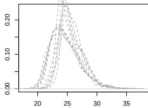
mean
