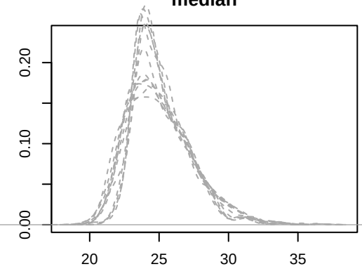
median
