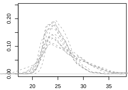
RLR
