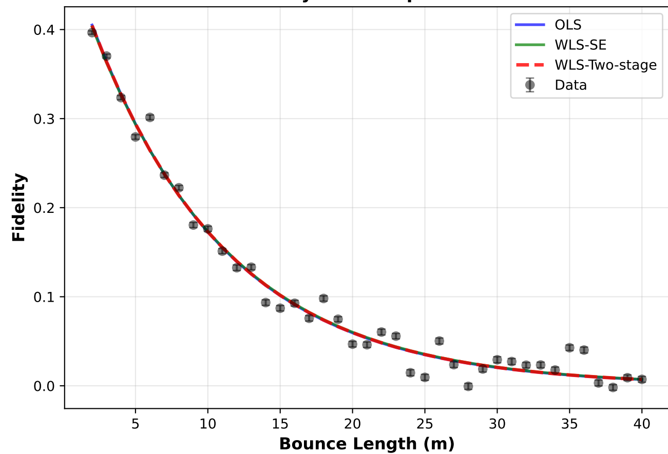
Decay Fits Comparison
