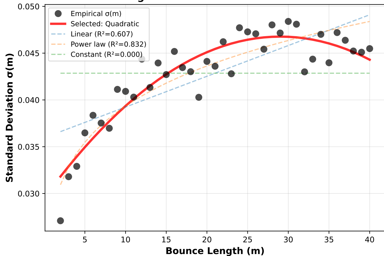
Estimation Precision Comparison
