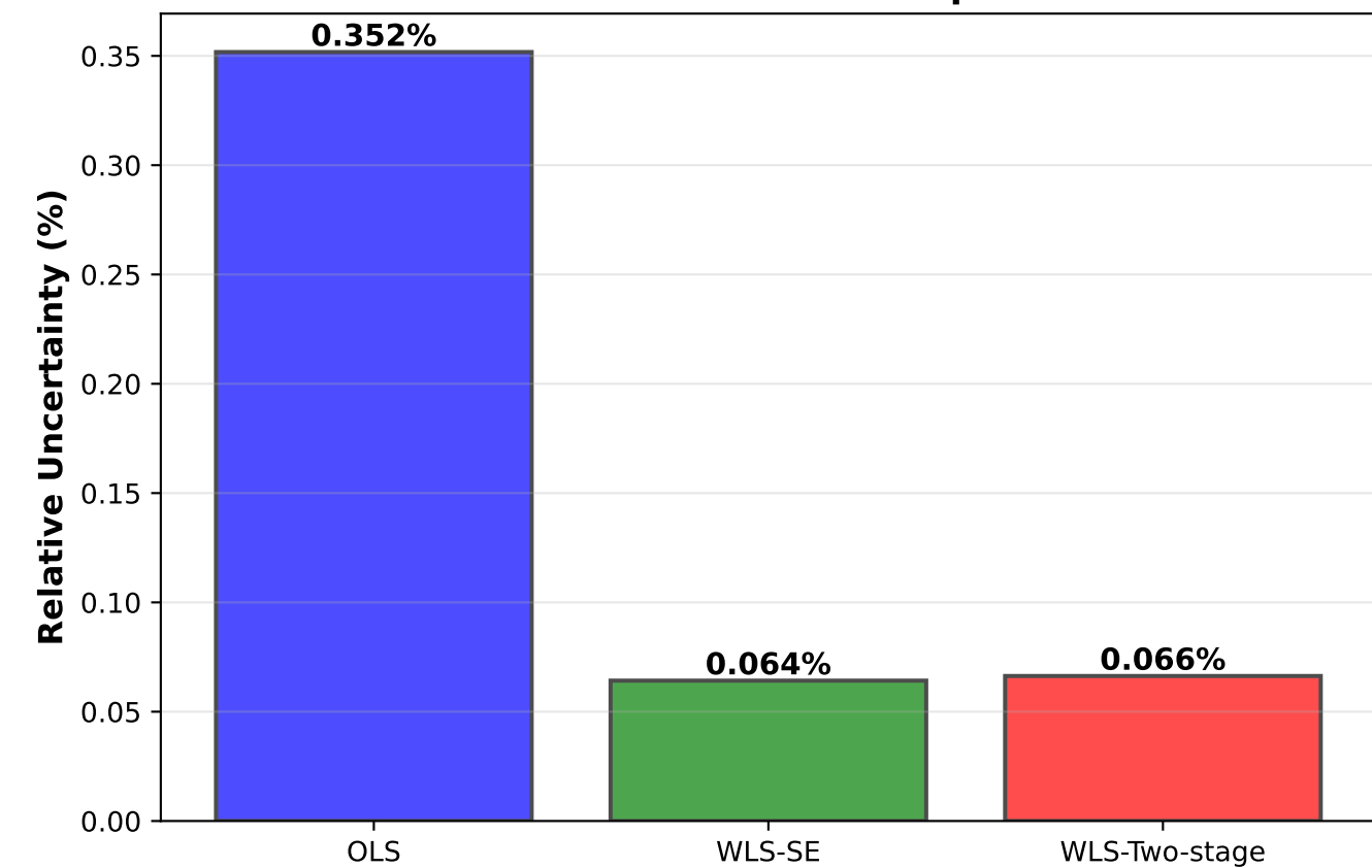
Estimation Precision Comparison
