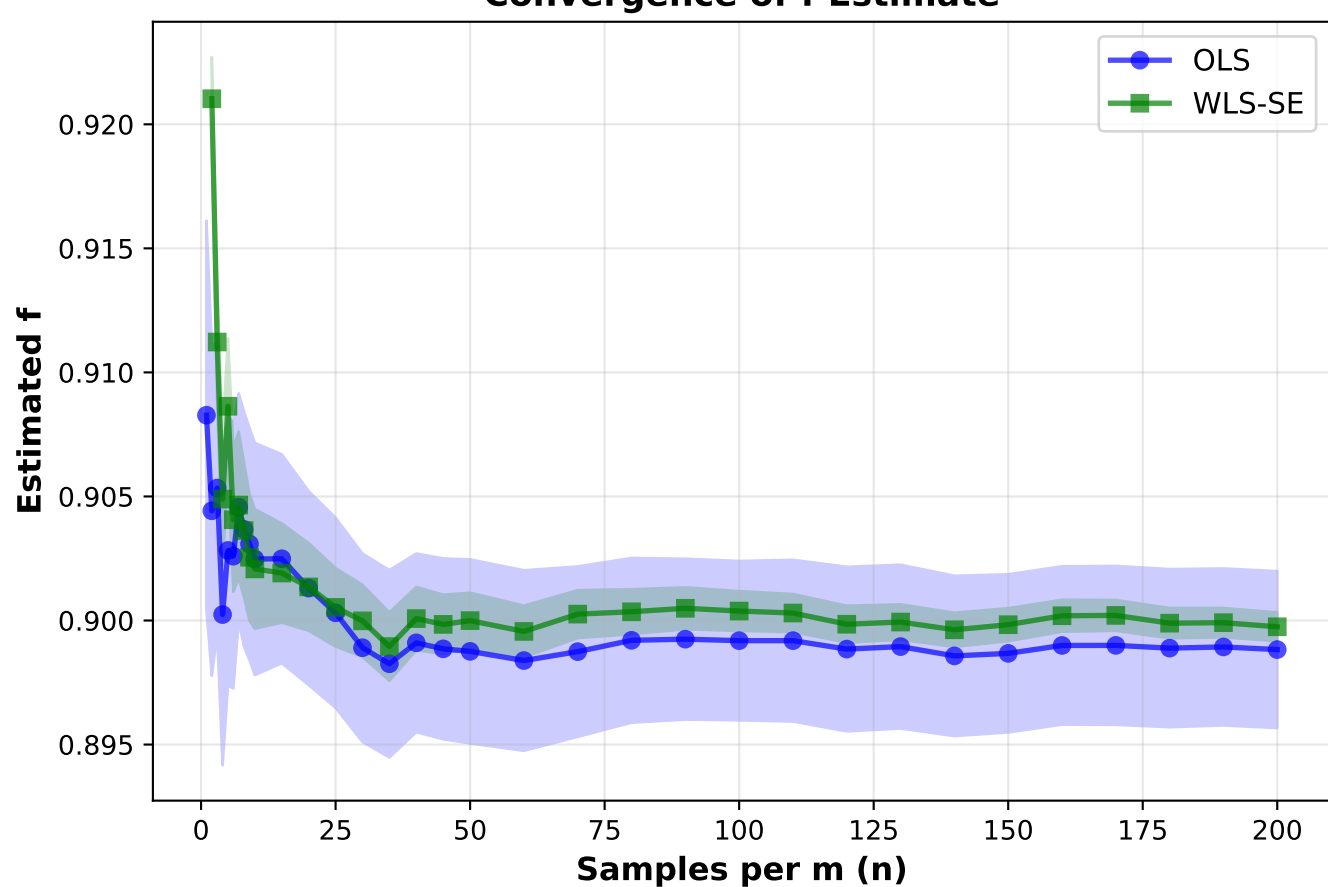
Convergence of f Estimate
