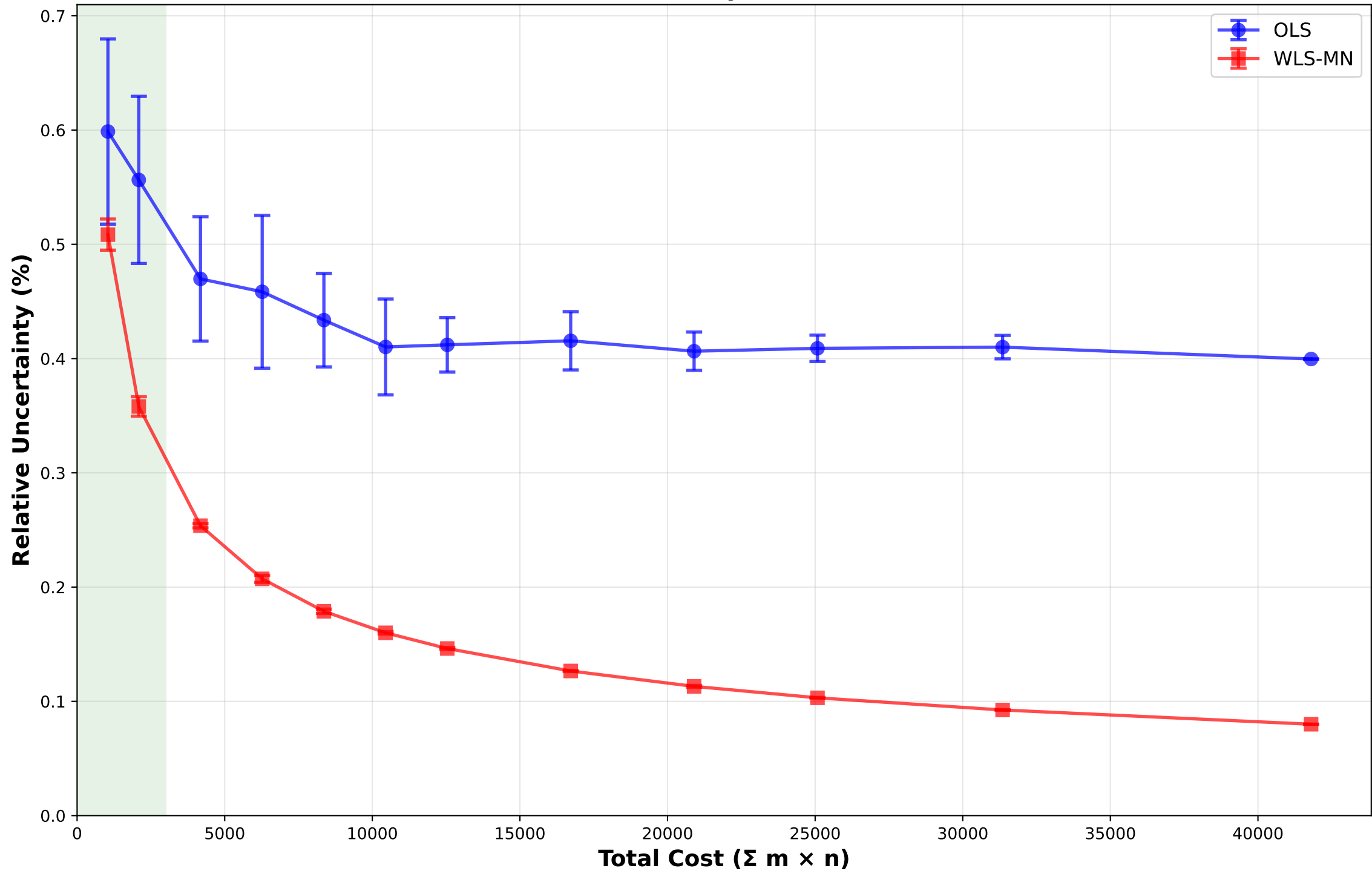
Cost vs Uncertainty: OLS vs WLS-MN
