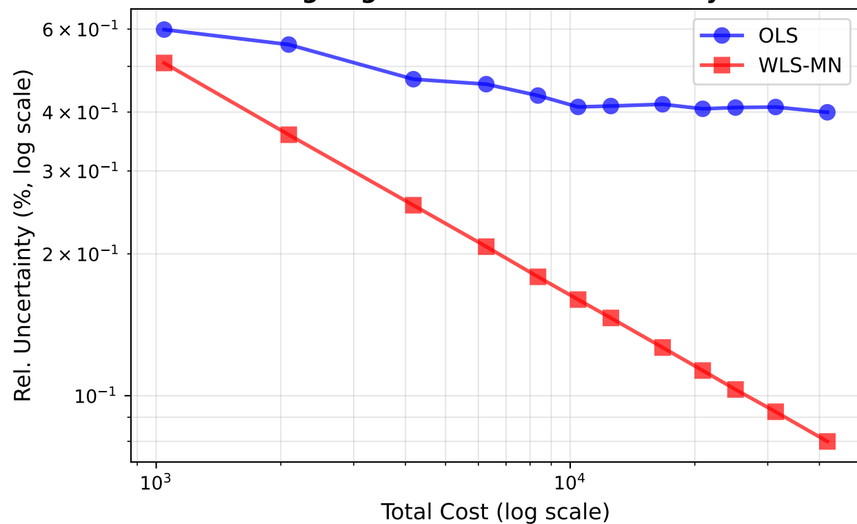
Log-Log Plot: Cost vs Uncertainty
