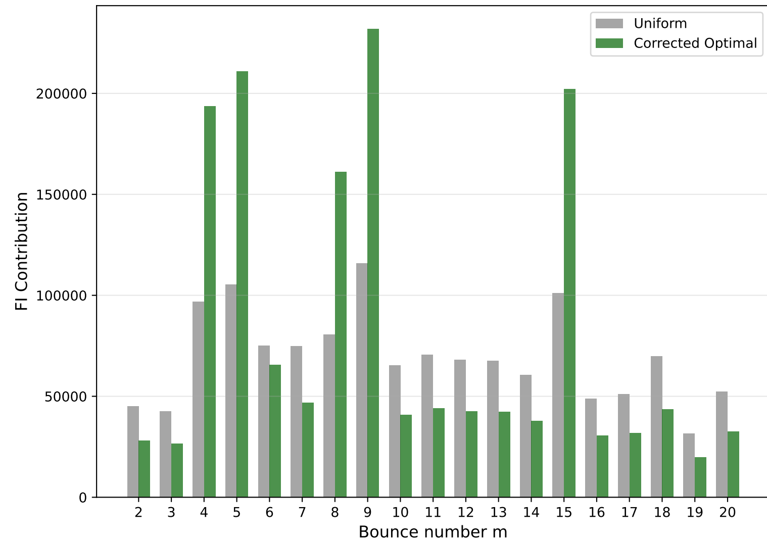
Fisher Information Contribution
