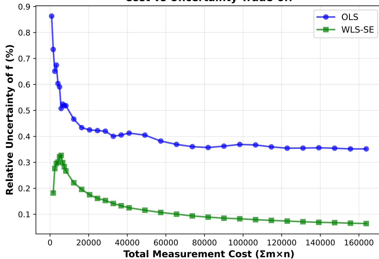
Samples vs Uncertainty
