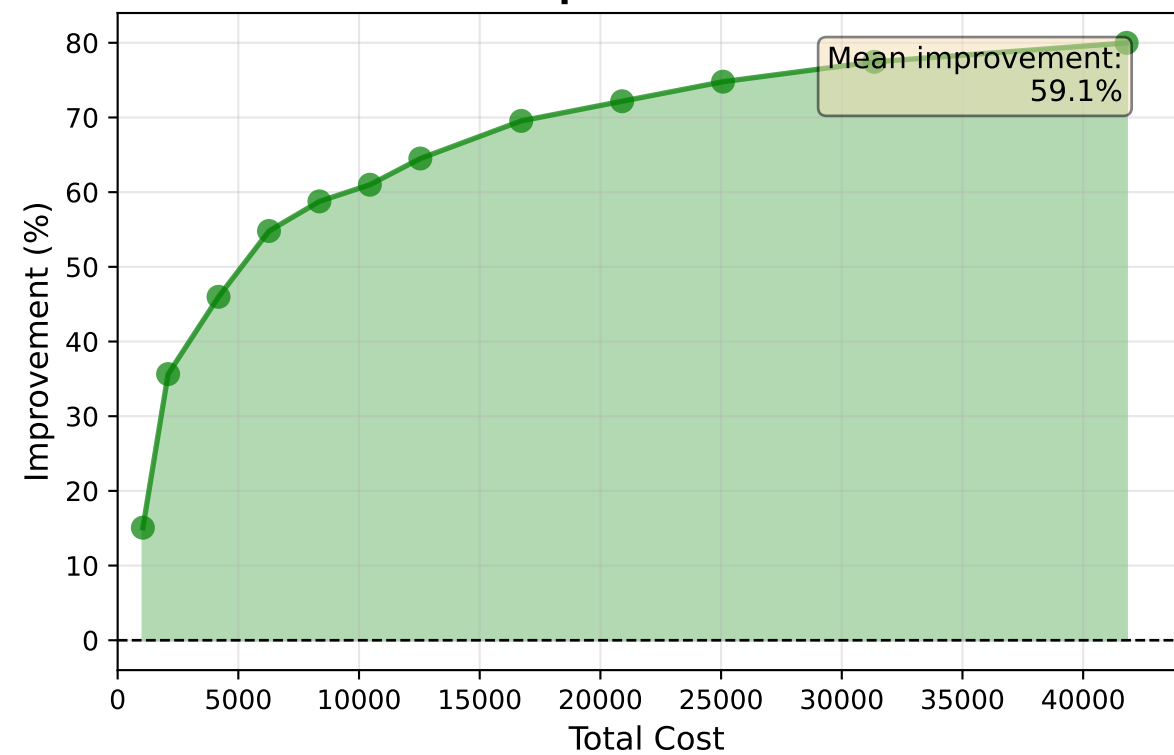
WLS-MN Improvement over OLS
